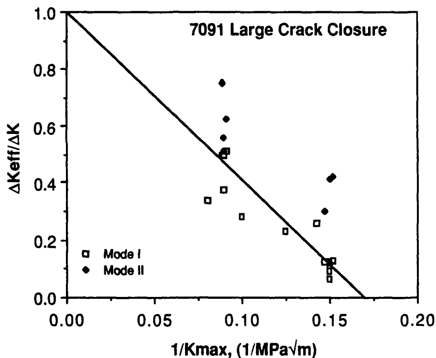
Fig. 1 Fatigue crack closure for the powder metallurgy aluminum alloy 7091, as determined from local measurements of opening load [2]. Note that \Delta K_{\text{eff}} for Mode II is larger than that for Mode I.
