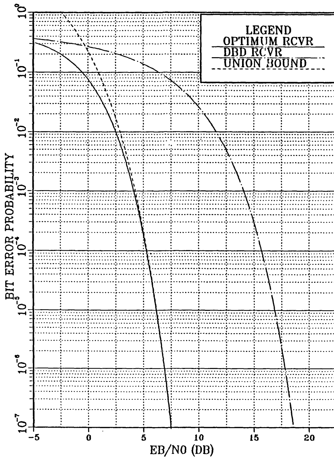
Figure 19. 16FSK/QPSK Bit Error Performance ( k = 6 bits/symbol)
