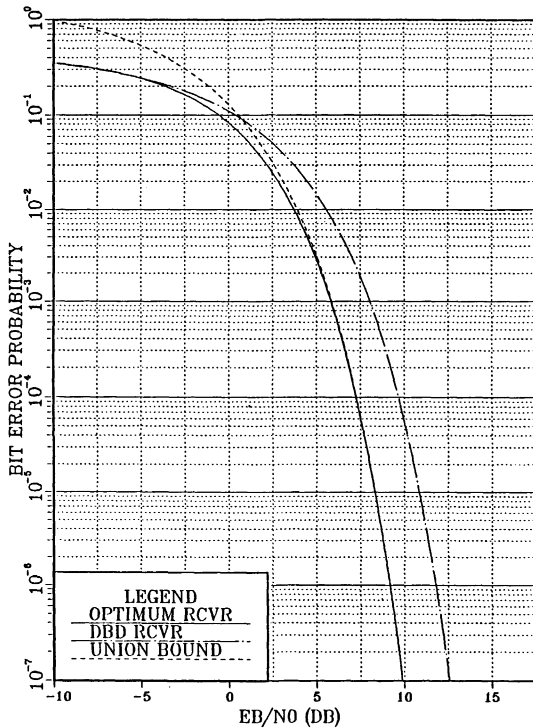
Figure 16. 2FSK/QPSK Bit Error Performance ( k = 3 bits/symbol)
