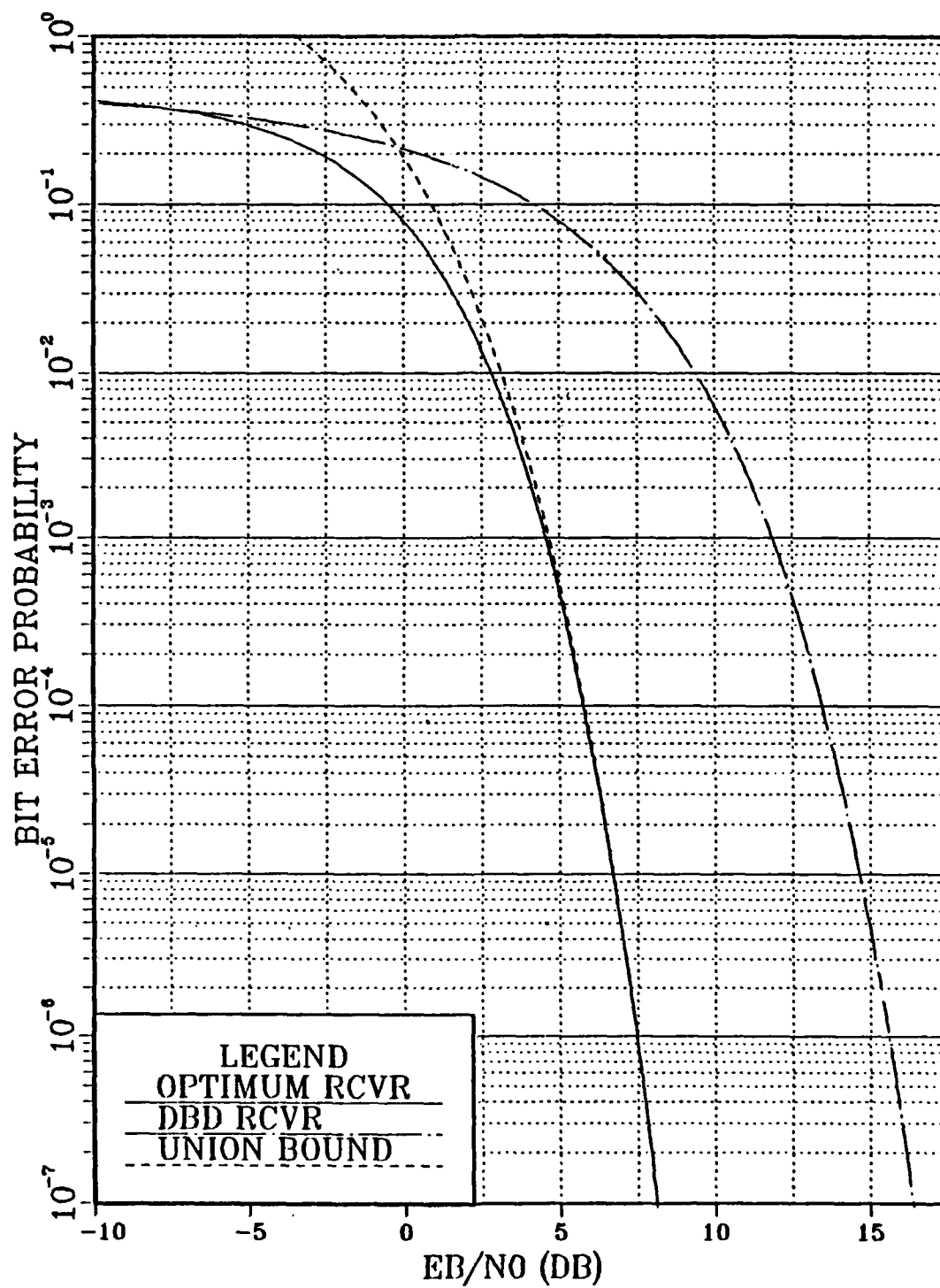
Figure 18. 8FSK/QPSK Bit Error Performance ( k = 5 bits/symbol)
