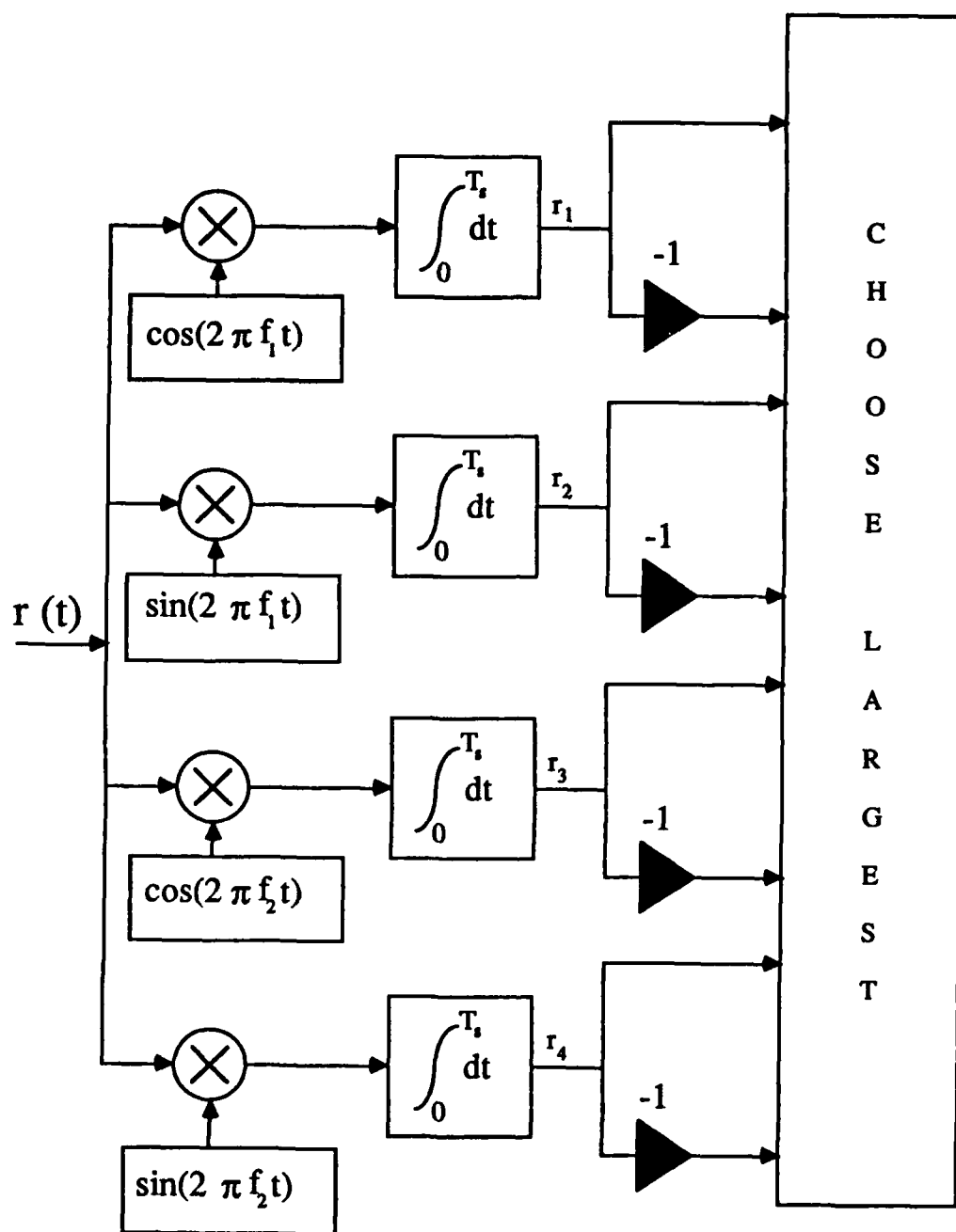
Figure 12. Diagram of Correlation Receiver for 2FSK/QPSK
