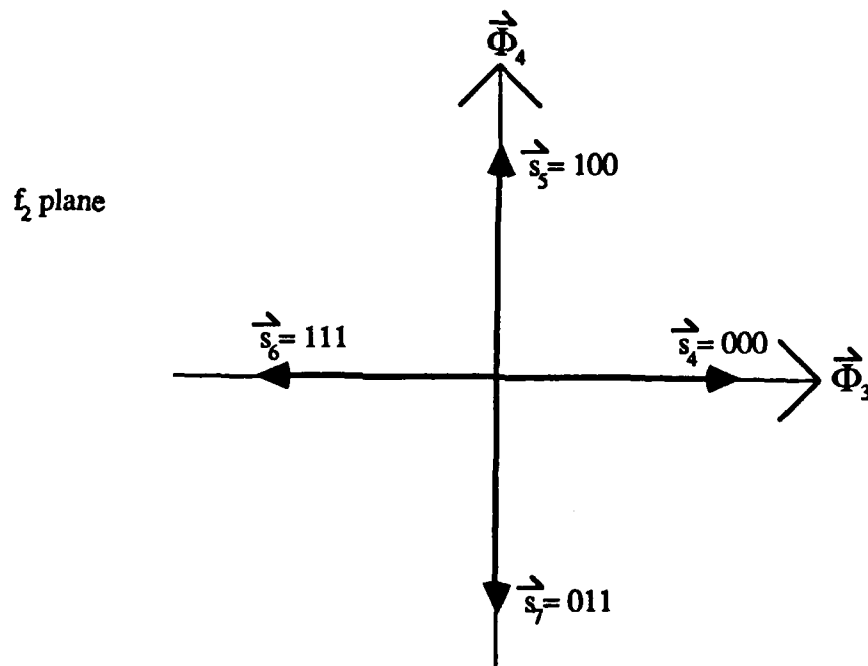
Figure 10. Vector Representation of 2FSK/QPSK
