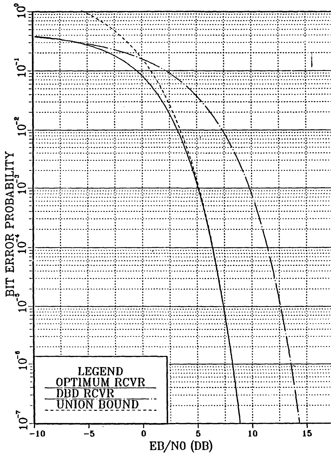
Figure 17. 4FSK/QPSK Bit Error Performance ( k = 4 bits/symbol)
