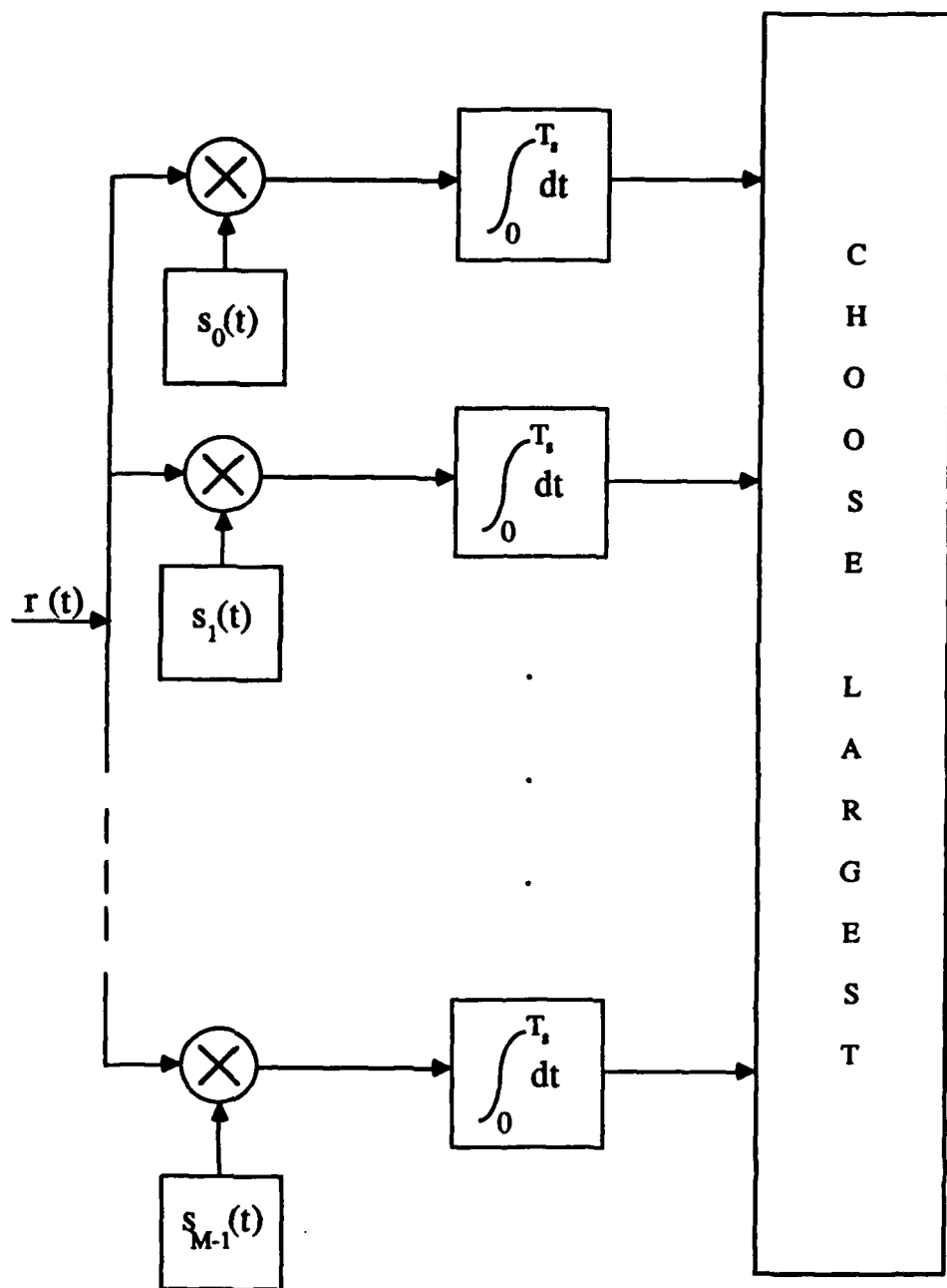
Figure 4. Receiver Structure for M-ary PSK
