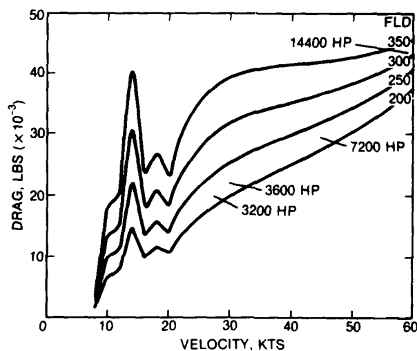
Fig. 15. SES-200 speed/power
