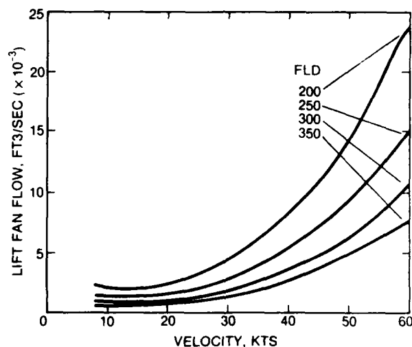
Fig. 17. SES-200 lift flow
