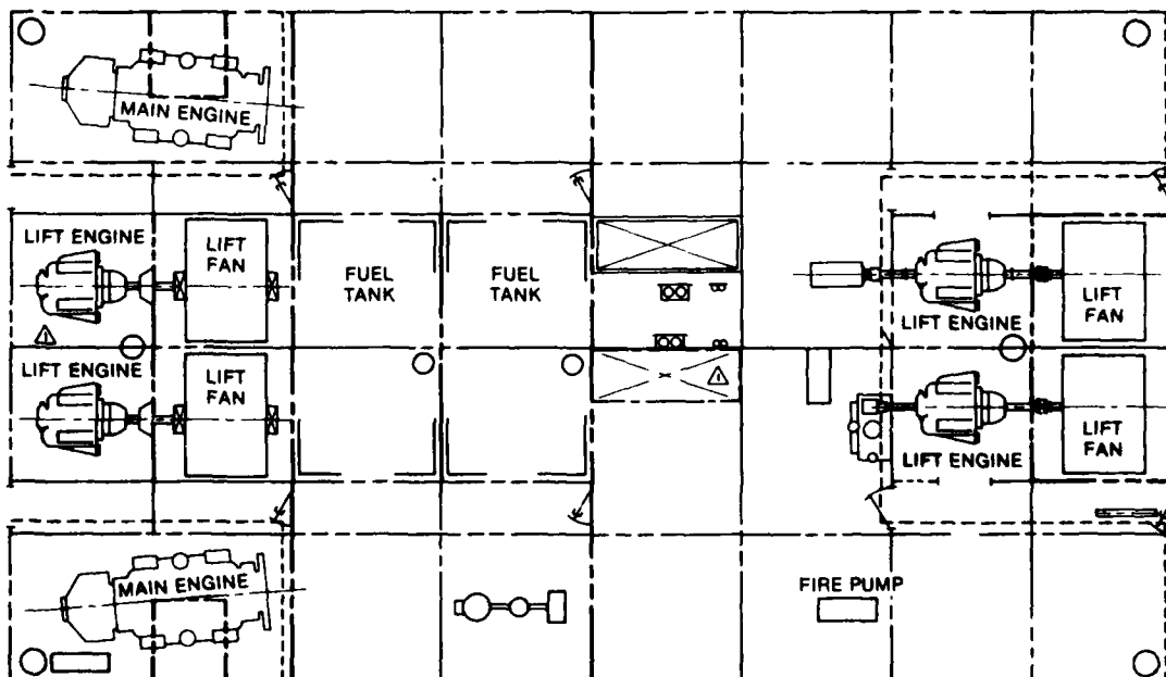
Fig. 21. SES-200 lift system
