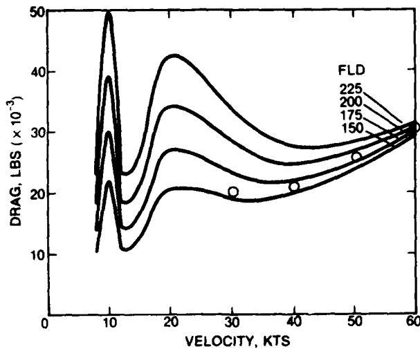
Fig. 18. WSES full-load displacement
