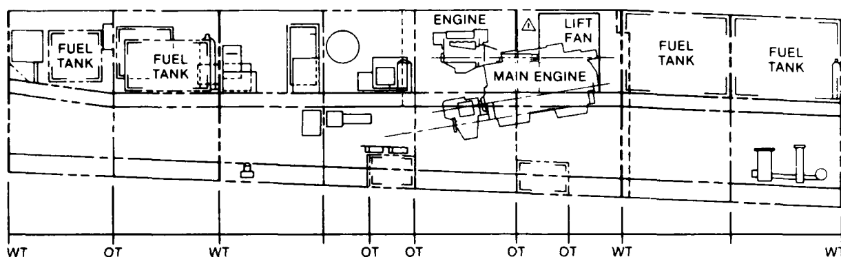
Fig. 22. Diesel propulsion system
