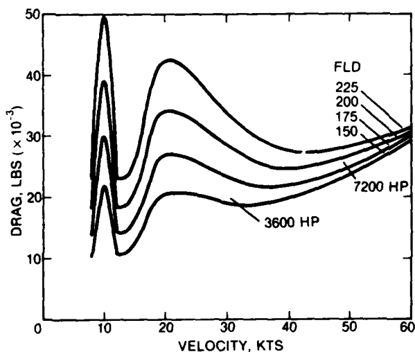
Fig. 14. WSES speed/power
