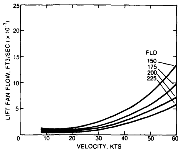
Fig. 16. WSES lift flow
