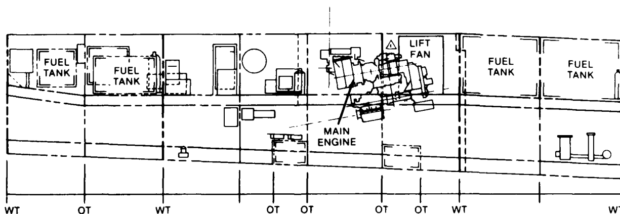
Fig. 23. Gas turbine propulsion system
