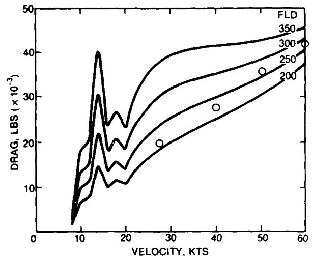
Fig. 19. SES-200 full-load displacement
