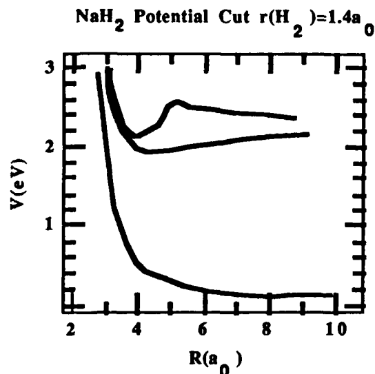
Figure 3. \text{Na} + \text{H}_2 potentials for \text{C}_{2v} approach of Na.
