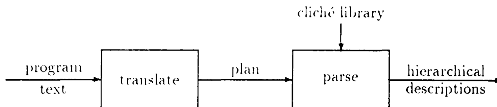
Figure 5. Architecture of the prototype recognizer.
