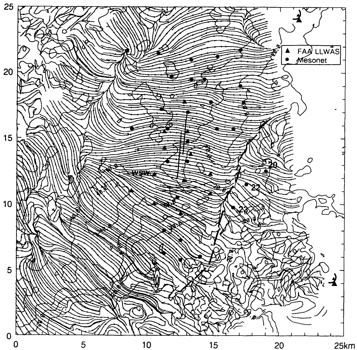
Figure VI-7b. Dual Doppler plot of the streamline and reflectivity field at 0026:14 UTC on 26 August 1987. The MBIdiv line is clearly evident in the northwest quadrant and the dashed line denotes the gust front boundary. Both of these wind shear lines are moving from the northwest toward the southeast.
