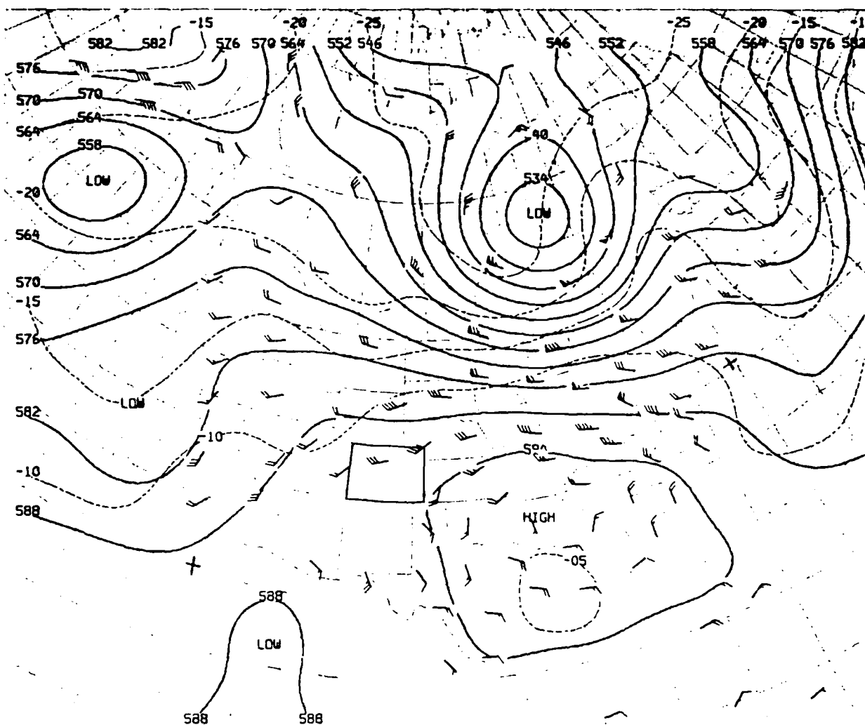
500-MILLIBAR HEIGHT CONTOURS AT 7 O' CLOCK E.S.T.
