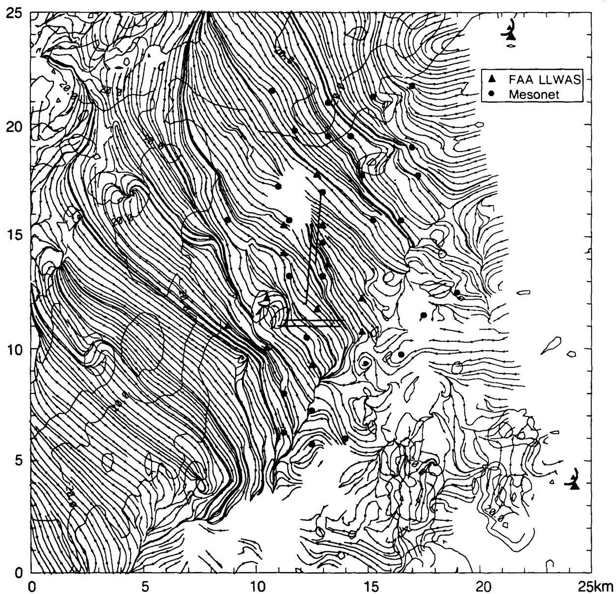
Figure V-11b. Dual Doppler plot of the streamline and reflectivity field at 2219:56 UTC on 21 August 1987.
