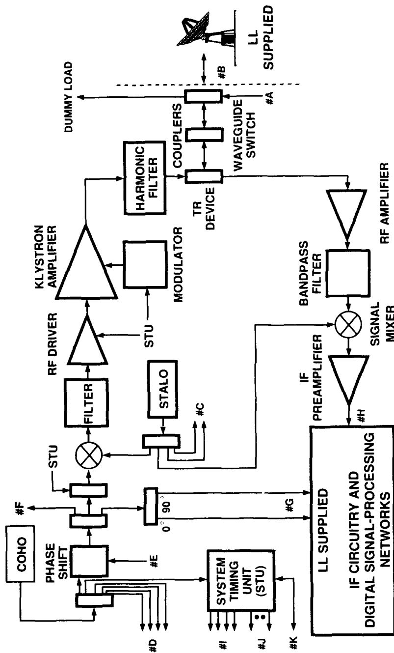
Figure 11-10. C-band transmitter/receiver subsystem.
