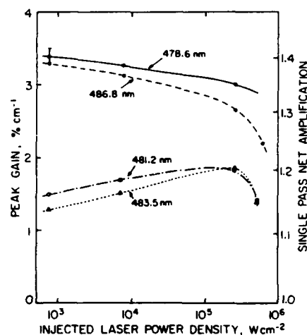
Fig. 11. Peak gain dependence on injected power density of the probe laser beam at various discrete wavelengths (Fig. 10); the electron-beam pumping energy was 95 J/l.
