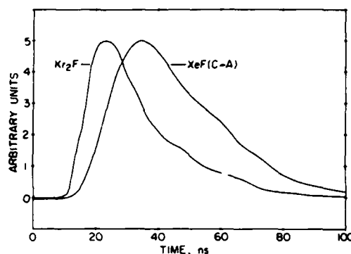
Fig. 8. Normalized temporal evolution of the Kr_2F and XeF(C \rightarrow A) fluorescence spectra for the conditions of Fig. 4(d) and Fig. 7.
