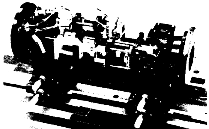
Fig. 16. Photograph of a compact 5 in. real-time SDF/CGH-based multi-channel correlator (courtesy D. Fetterly, General Dynamics-Pomona).
