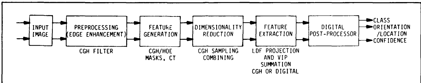
Fig. 3. Block diagram of a general feature extractor pattern recognition system with emphasis on the use of CGHs.
