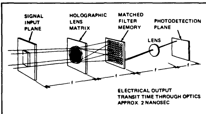
Fig. 15. Optical correlator with space-multiplexed MSFs using a CGH point hologram to replicate the Fourier transform of the input object. 22
