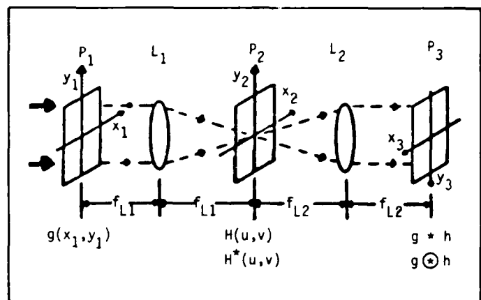
Fig. 2. Coherent optical matched spatial filter (MSF) frequency plane correlator.
