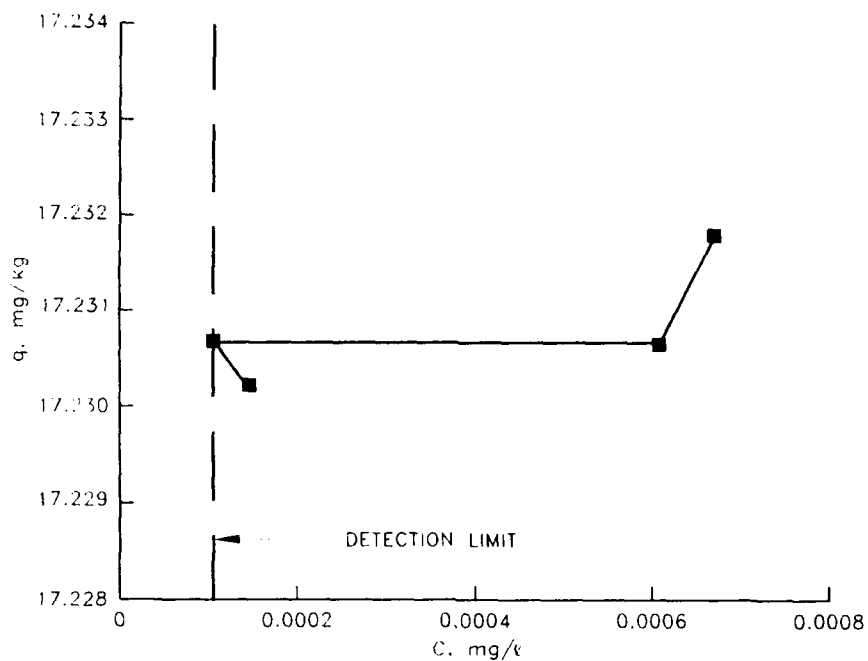
Figure B49. Cadmium desorption isotherm for hot-spot sediment solidified/stabilized with 0.3 STC proprietary additive:1.0 wet sediment
