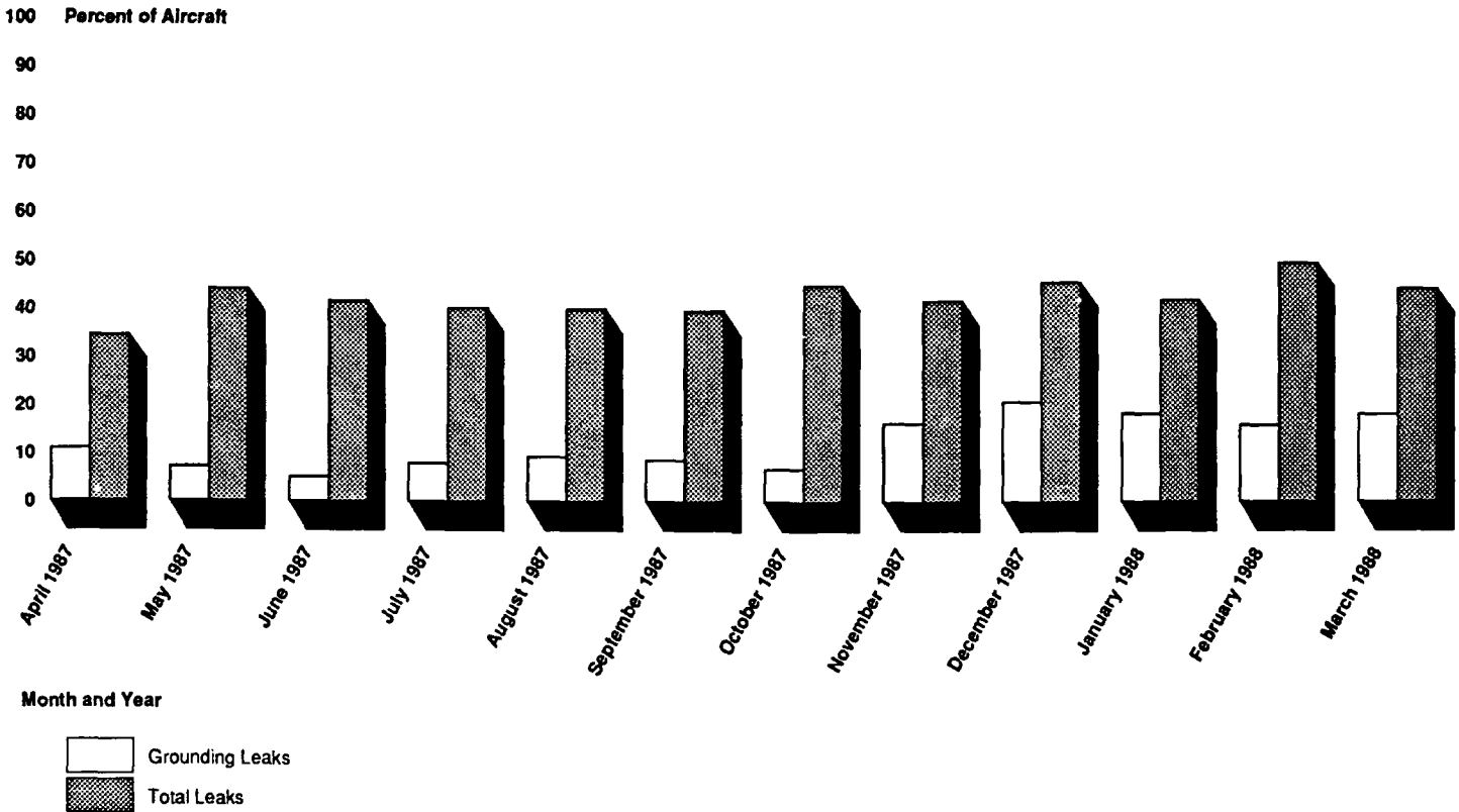
Figure 2.1: Percent of B-1Bs With Fuel Leaks From April 1987 to March 1988
