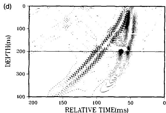
FIG. 2. TDPE solution generated with the Gaussian starter. The solid contours correspond to p > 0 . The dashed contours correspond to p < 0 . (a) r = 0 , (b) r = 50 m, (c) r = 100 m, (d) r = 500 m.
