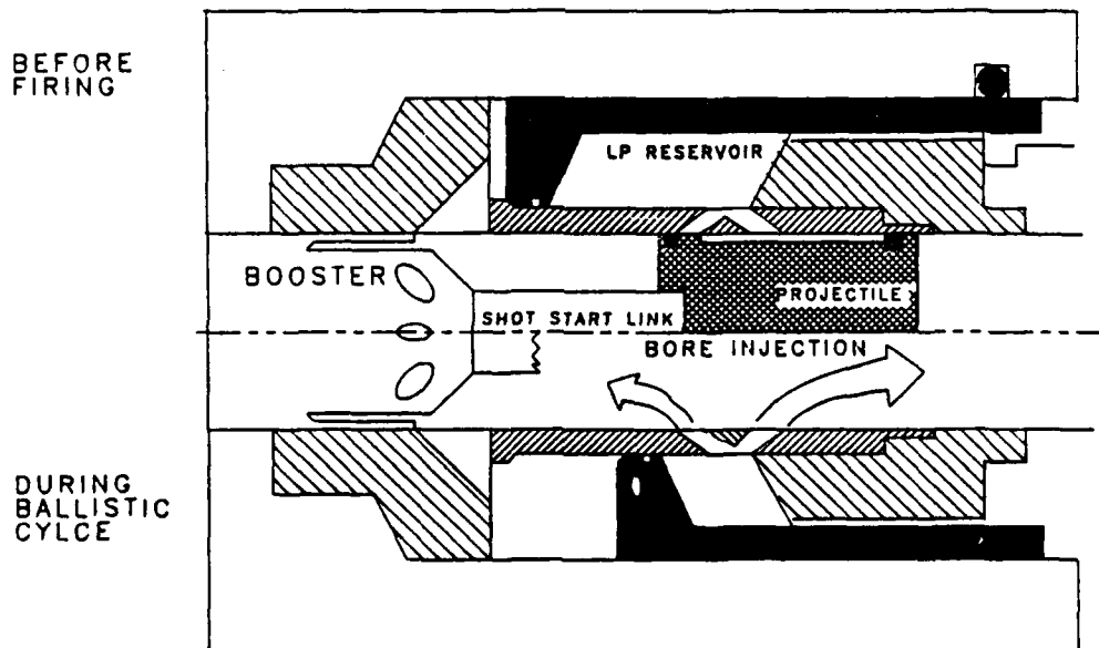
Figure 2. GE 30mm Reverse Annular Regenerative Liquid Propellant Gun.
