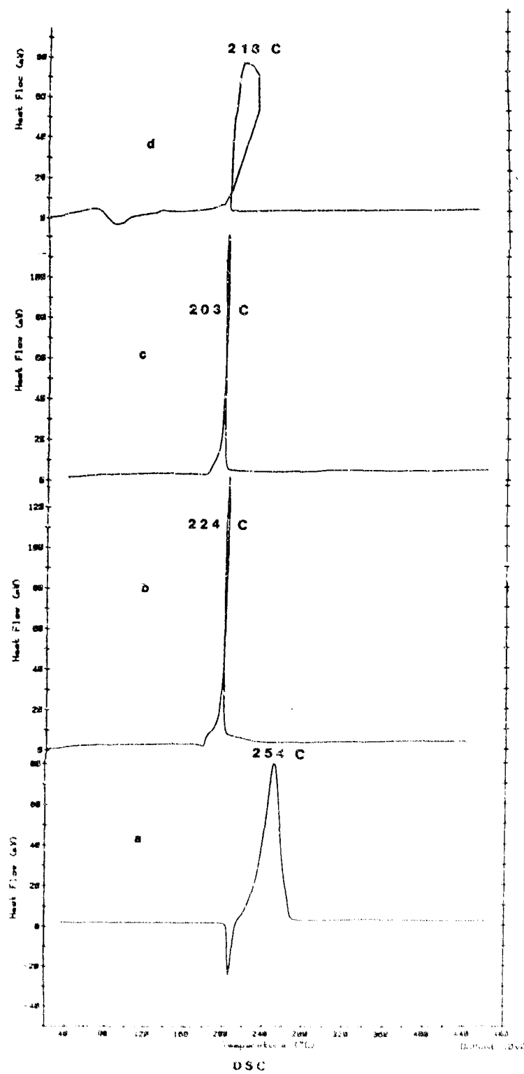
Figure 11. DSC Results for RDX (a) and Roughly 50:50 Mixtures of RDX with the Potassium Boron Salt (b), the TSA Boron Salt (c) and \text{NaBR}_6 (d)
