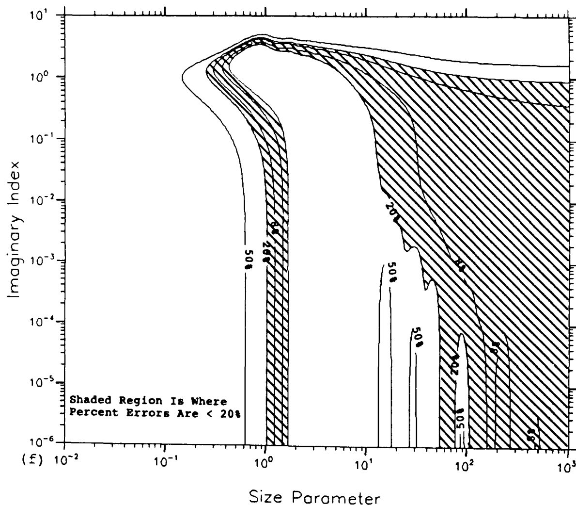
Figure 14. (continued) Percent Errors in Q_{abs} for the Approximation of (f) Bohren and Nevitt, for \bar{n} \cong 1.54
