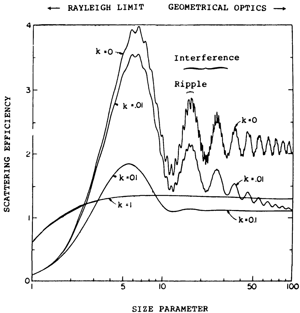
Figure 11. Mie Theory Calculations of Q_{sct} Showing the Interference and Ripple Structure as a Function of Size Parameter and k for Fixed n (= 1.33)
