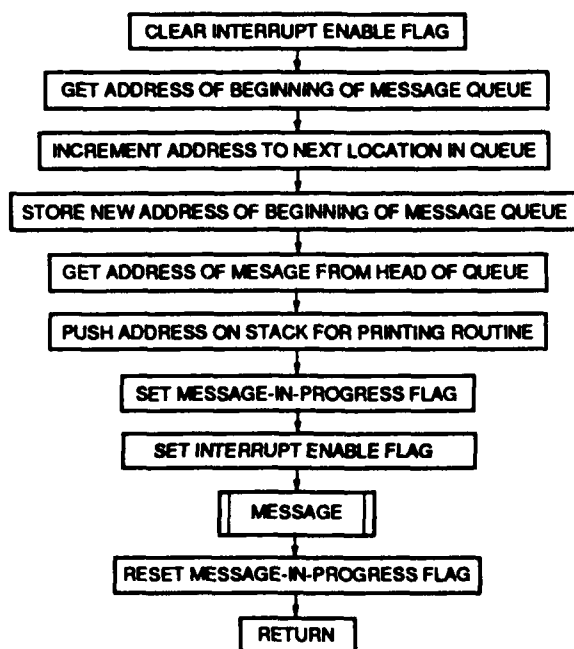
Figure 23. - Flow chart for message generation routine, MESGEN.
