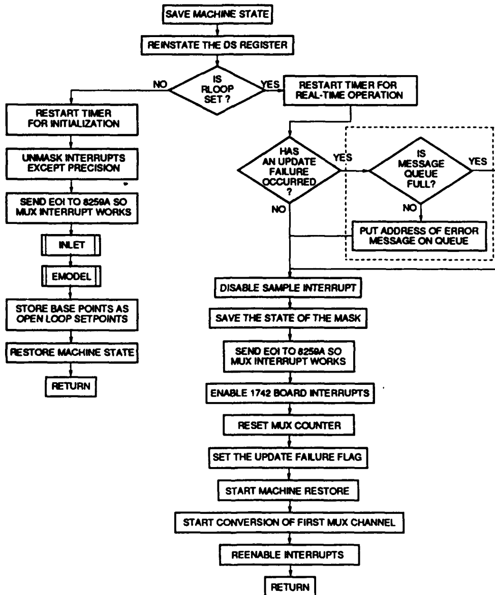
Figure 21. - Flow chart for timer interrupt service routine.
