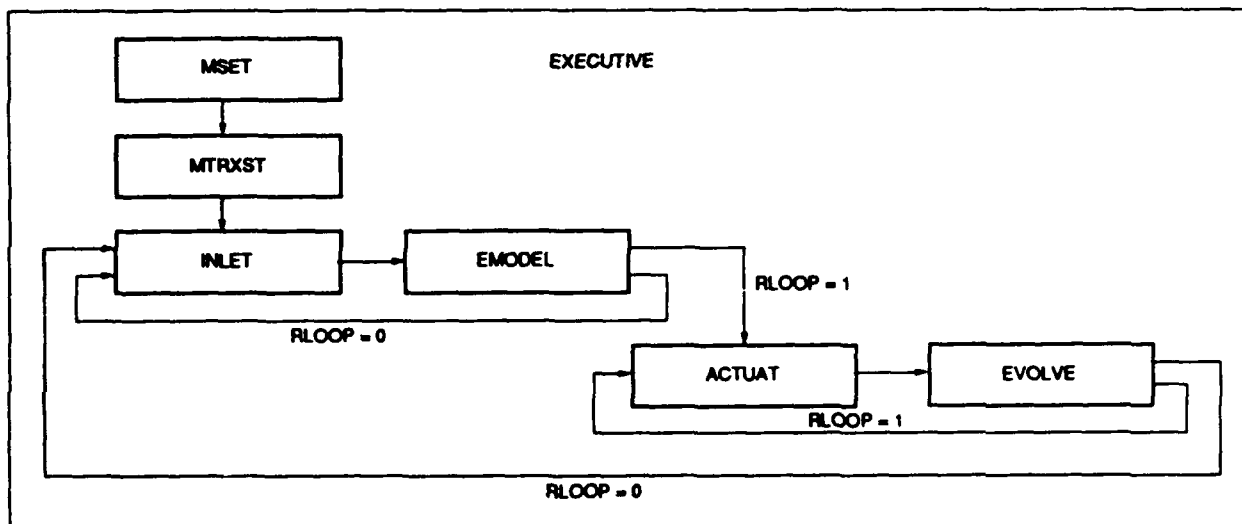
Figure 14. - Program flow.
