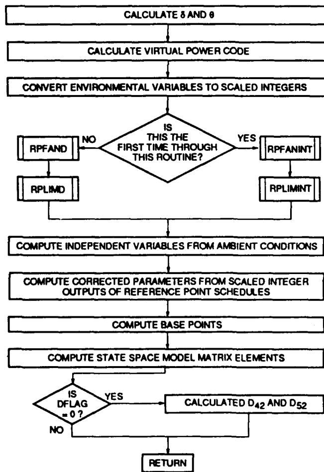
Figure 11. - Flow chart for routine to determine model at operating point, EMODEL.
