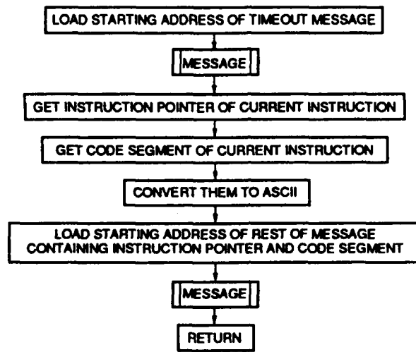
Figure 25. - Flow chart for system bus timeout interrupt service routine.
