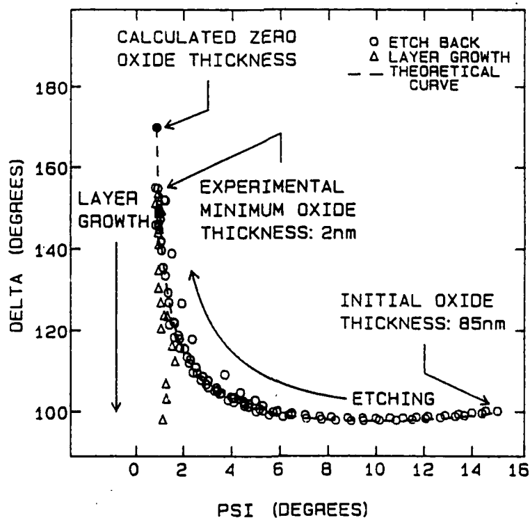
PSI vs. DELTA FOR HF ETCH EXPERIMENTS
