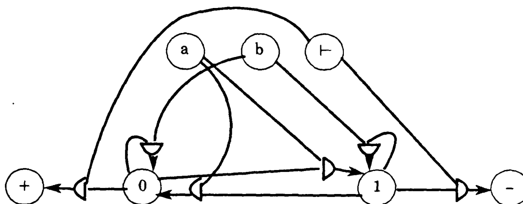
Figure 2: A connectionist parity network
