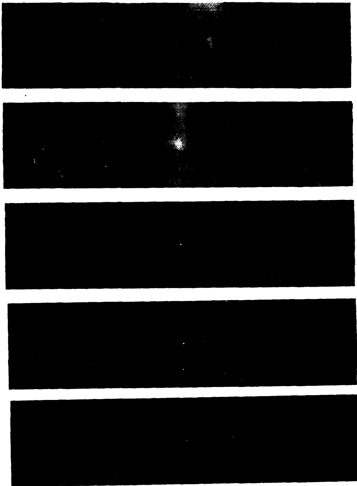
Figure 6: The cepstrum and related filters. a) A padded input image. b) The autocorrelation of the input image. Arrows show where the disparity peaks occur. c) Effect of taking the log of the power spectrum before inverting, i.e. the cepstrum. d) effect of taking the fourth root instead of the log. e) effect of taking the arc tangent.
