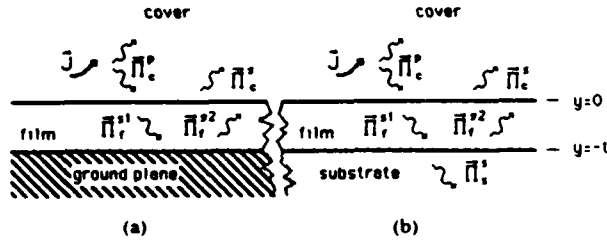
Fig. 3. Detail of potential components in (a) integrated electronic circuit and (b) integrated optical circuit.
