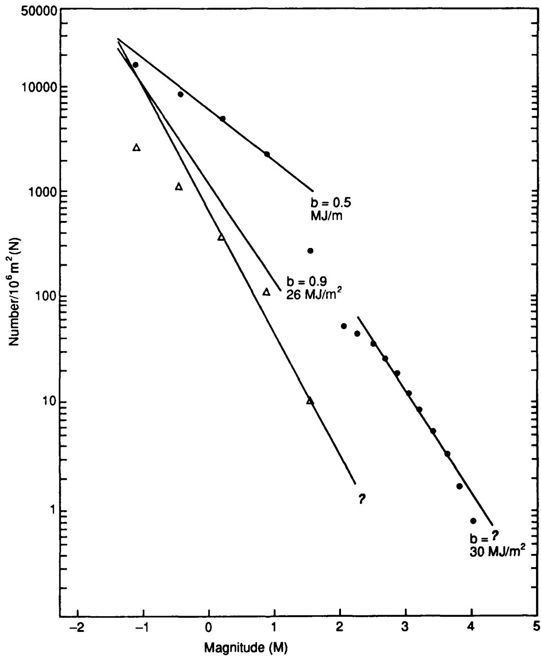
Figure 11. Plots of the logarithm of the cumulative number of seismic events greater than a given magnitude as a function of magnitude. The three lines in the top left are derived from underground seismic observations and that in the bottom right from a surface seismic station. (After Fernandez. 30 ) Note that the slope of these lines is a function of the spatial rate of energy release. 7
