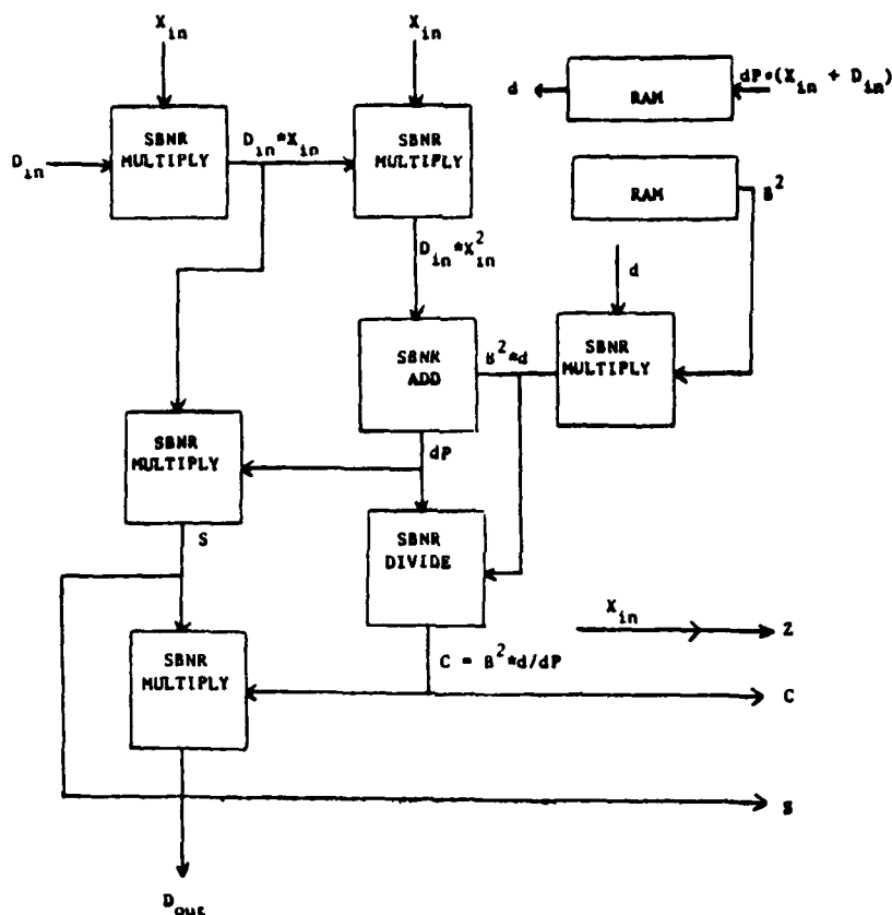
Figure 15 SBNR Boundary Cell Architecture
