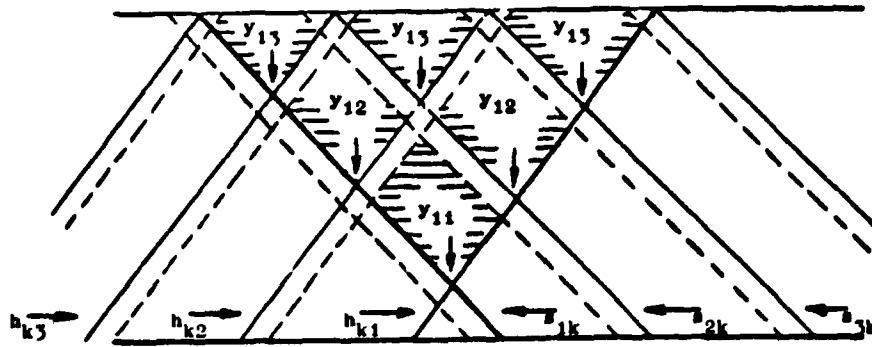
Figure 10 Partial Product Generation of Matrix x Matrix Multiplication
