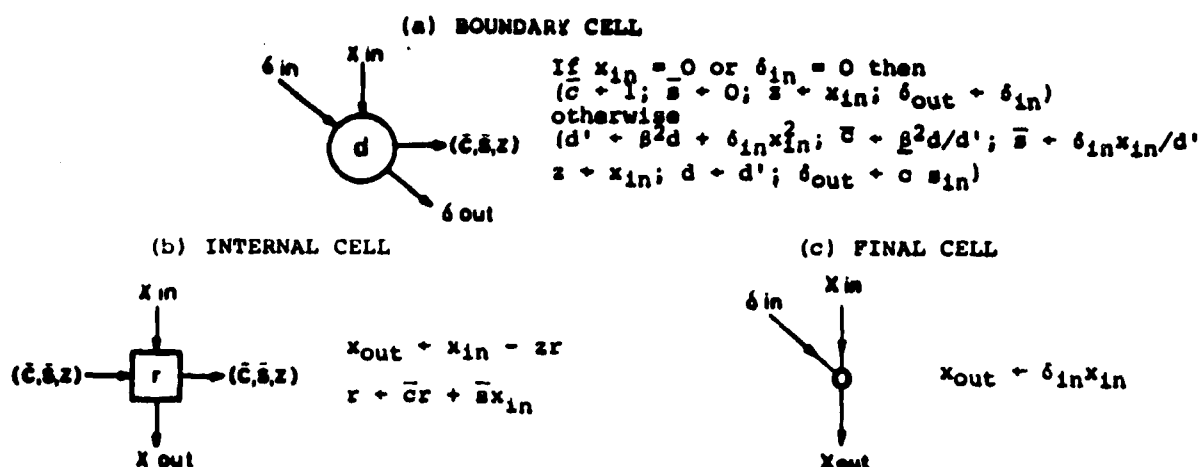
Figure 12 Cells Required for the Square-Root Free Givens Rotation
