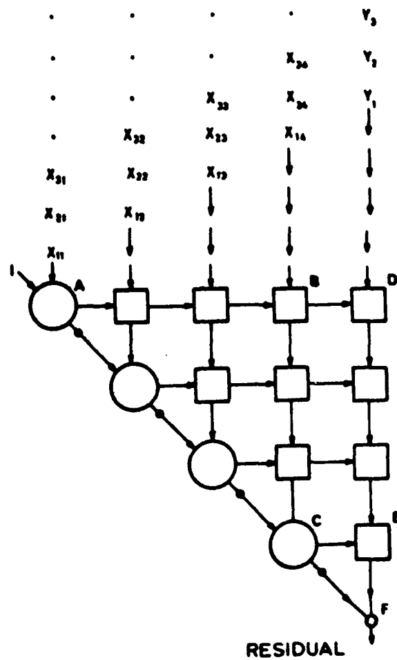
Figure 11 Systolic Array for Recursive Least-Squares Minimization
