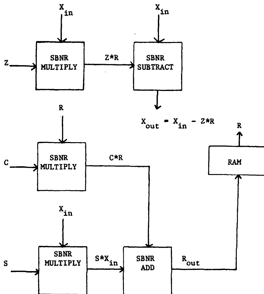
Figure 16 SBNR Internal Cell Architecture
