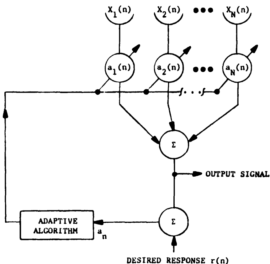
Figure 3a Adaptive Antenna
