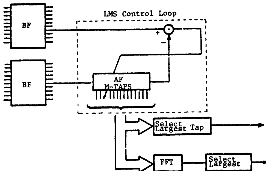
Figure 20a LMS Time Domain Adaptive Tracker
