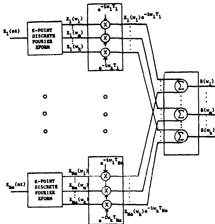
Figure 22a Frequency Domain Adaptive Beamformer
