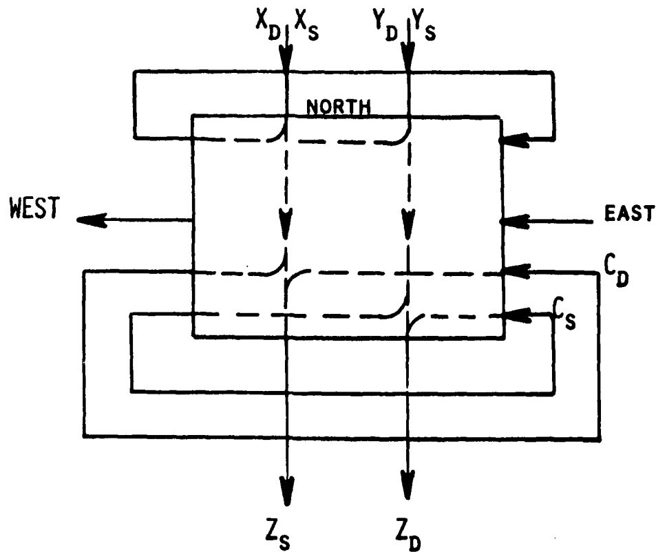
Figure 8 Primitive Cell (Internal Data Flow)
