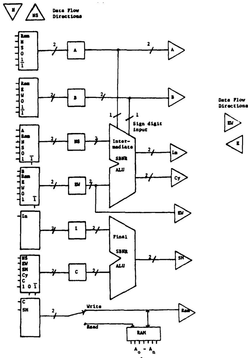
Figure 14 An SBNR Primitive Cell for a 2-D Mesh Connected Array
