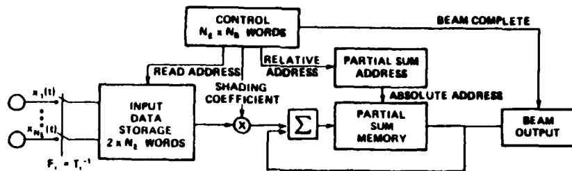
Figure 23 Discrete-Time, Partial-Sum Beamformer
