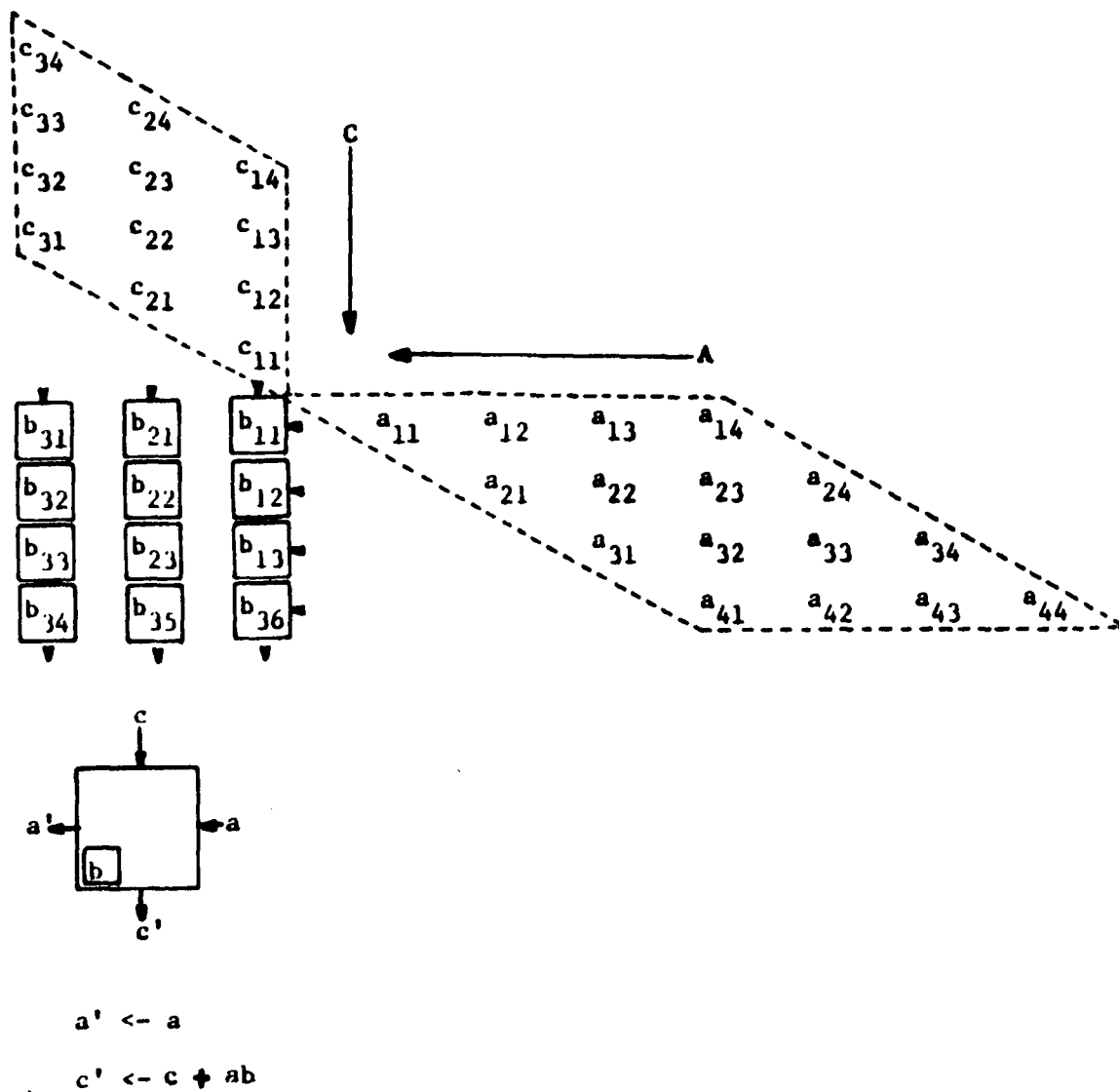
Figure 6b Matrix x Matrix Multiply Array Using Static Coefficients
