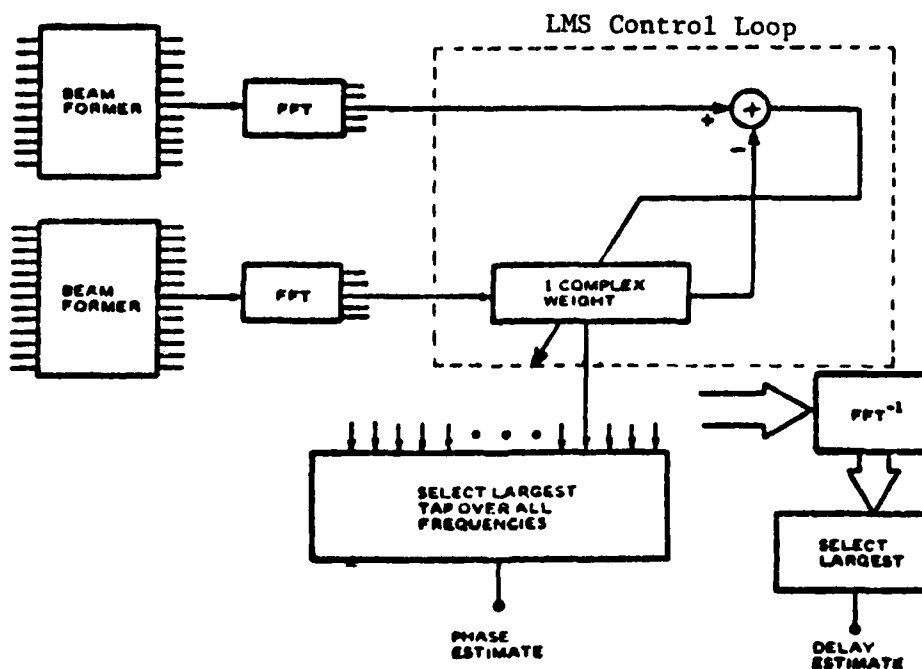
Figure 20b LMS Frequency Domain Adaptive Tracker
