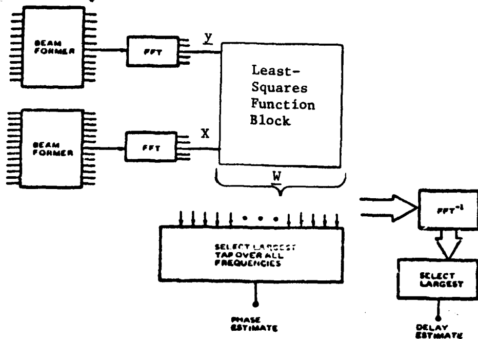
Figure 21b Least-squares Frequency Domain Adaptive Tracker
