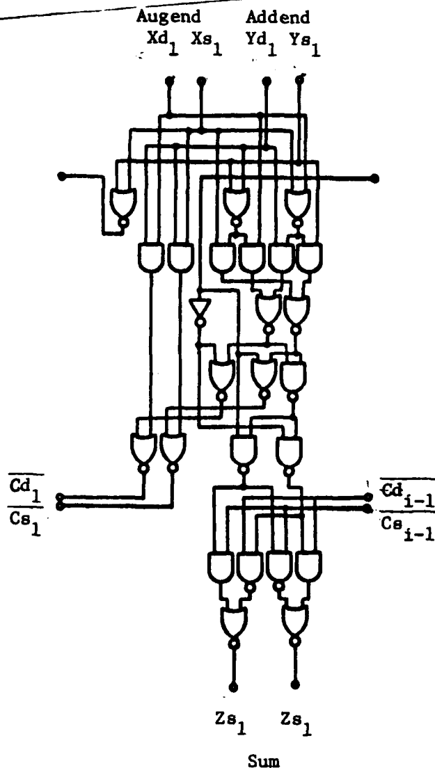
Figure 7 Primitive Bit-Serial Cell
