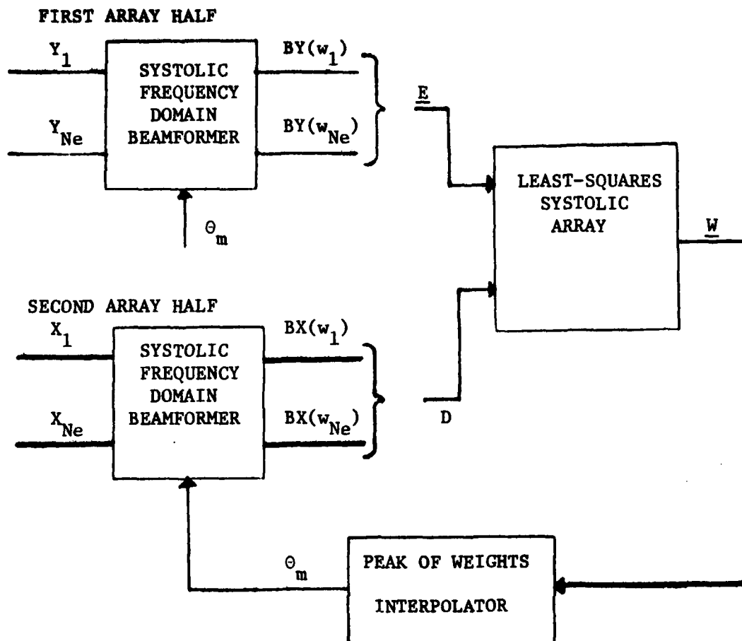
Figure 22b Frequency Domain Adaptive Beamformer and Tracker
