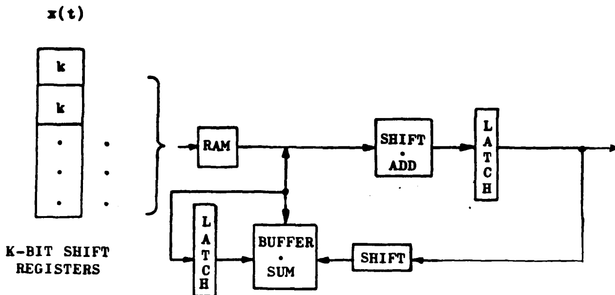
Figure 18 Distributed Arithmetic Primitive Element Architecture
