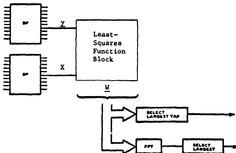
Figure 21a Least-squares Time Domain Adaptive Tracker
