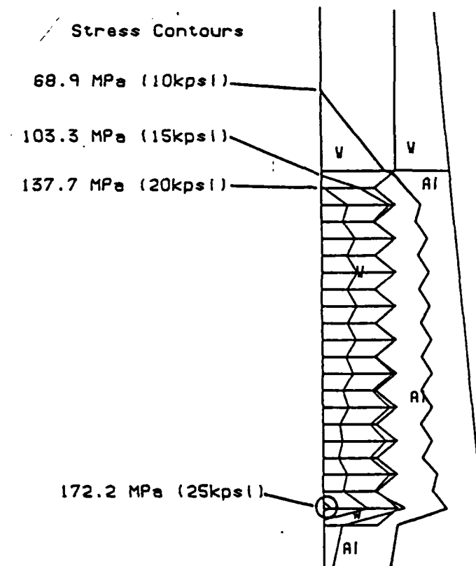
Figure 9. Predicted stresses for 10 mm model for a 31,000 g load.
