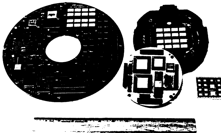
Figure 5.3-4 High-Speed, Miniature Processors
