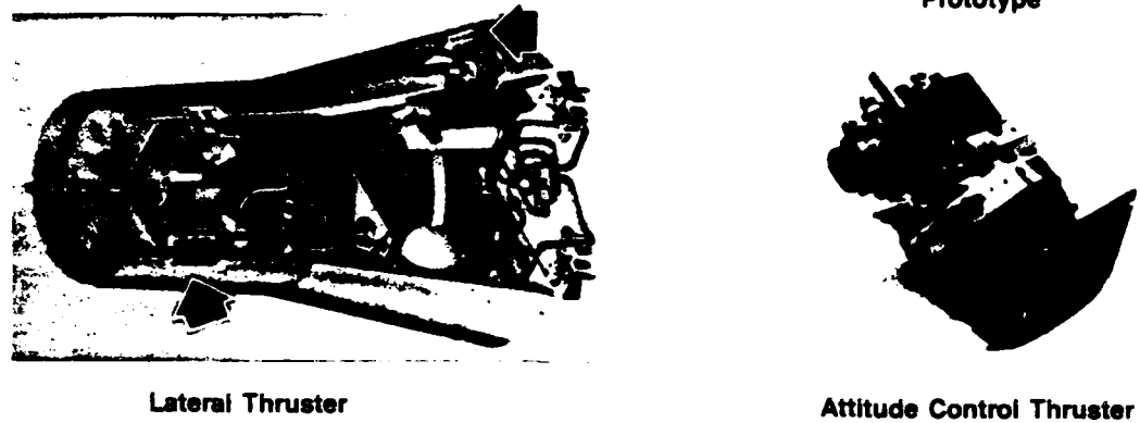
Figure 5.5-4 Compact, Fast-Response Control Thrusters for HEDI
