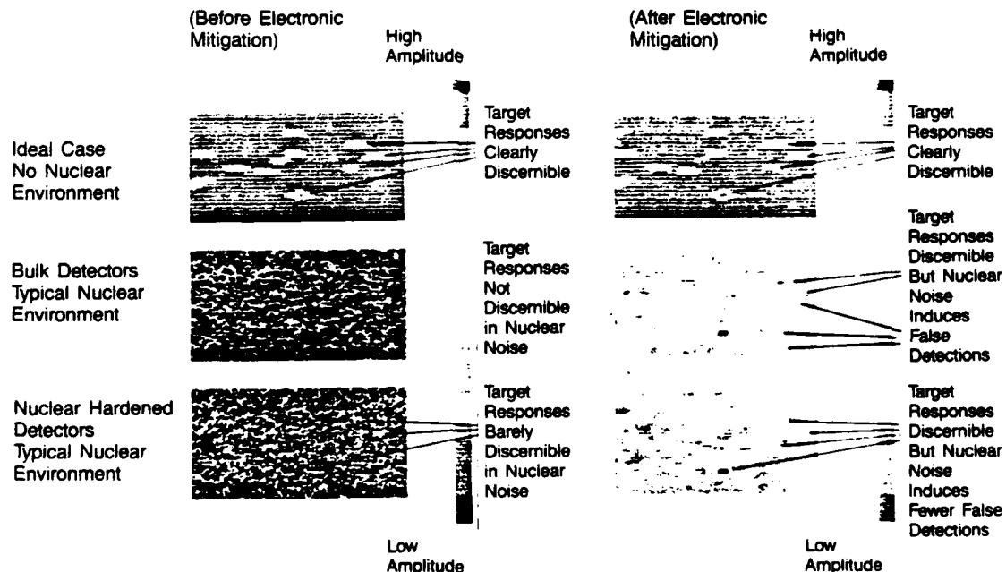
Figure 6.1-5 Infrared Sensor Imagery (Before and After Electronic Mitigation)
