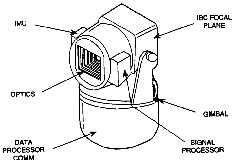
Figure 5.2-2 GSTS Payload
