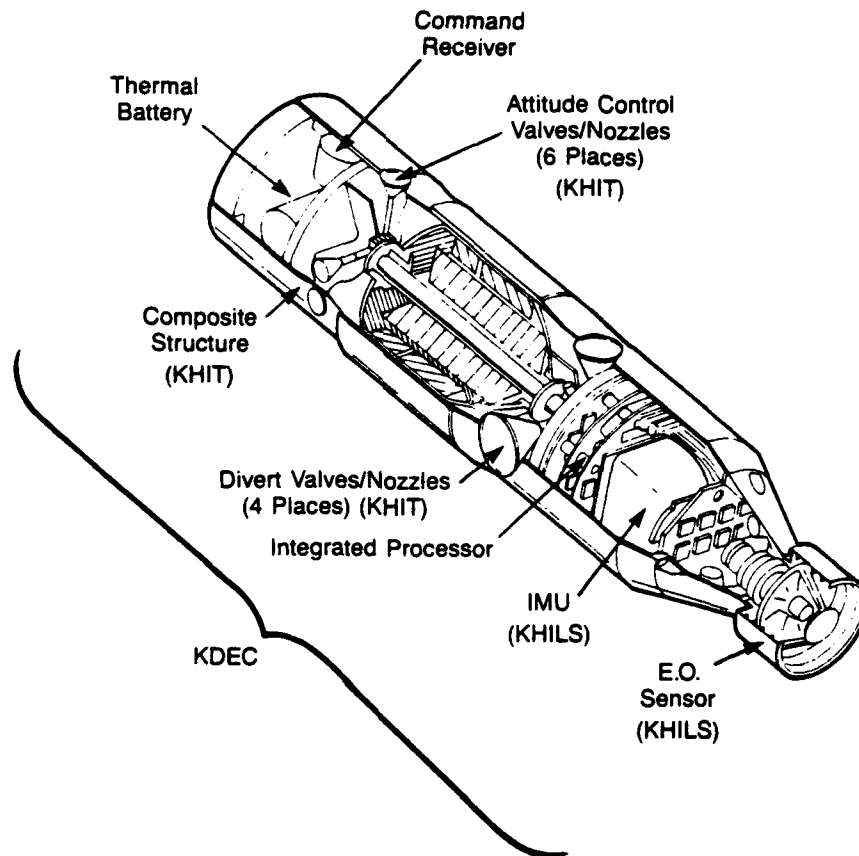
Figure 6.3-8 Interceptor Validation
