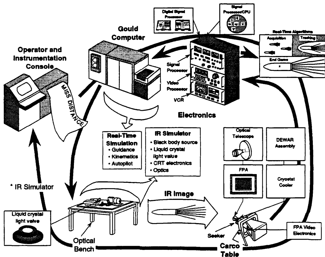
Figure 6.3-10 KHIL Testing
