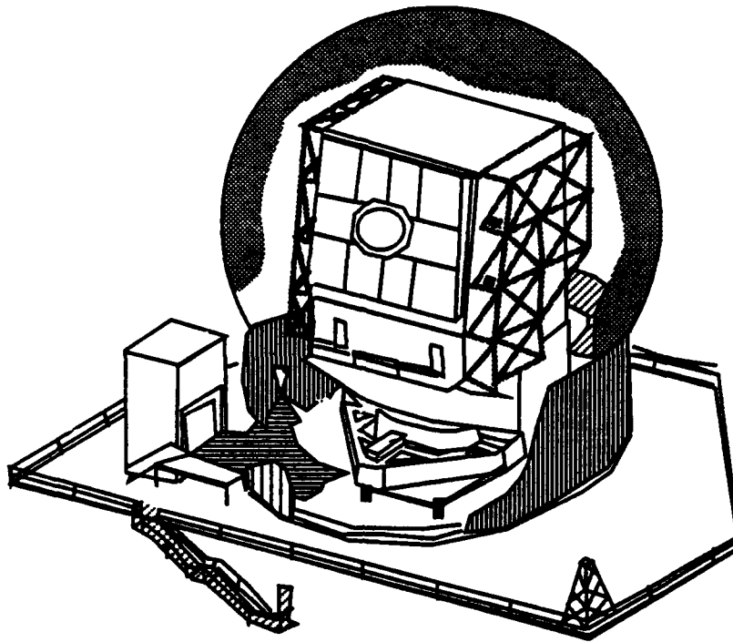
Figure 5.2-4 GBR-X
