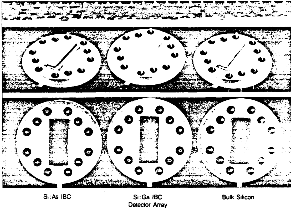
Figure 6.1-3 SEER/PATHS IRA FPA Hybrids
