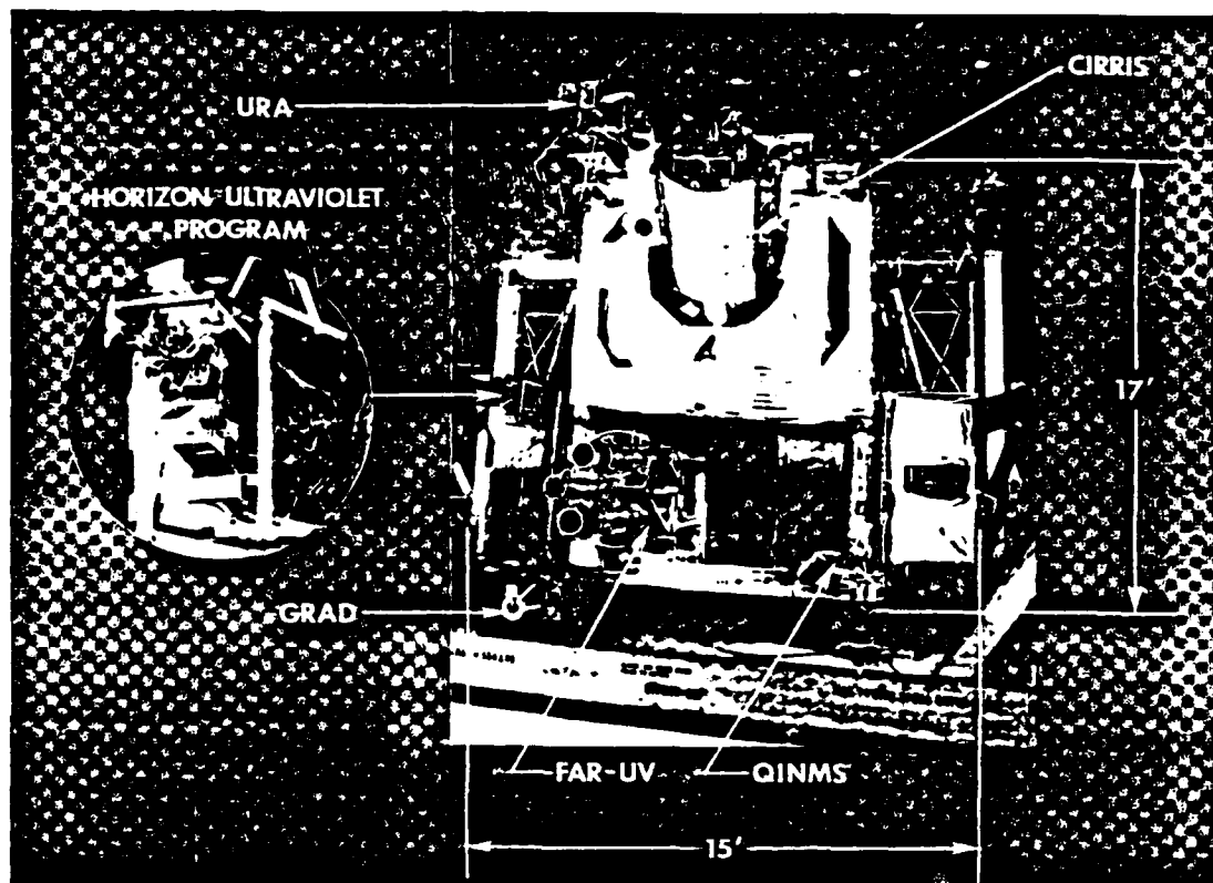
Figure 6.1-12 CIRRIS 1A
