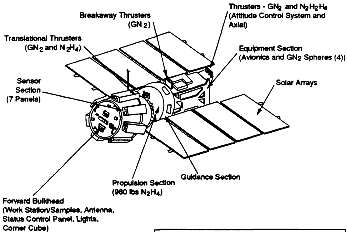
Figure 6.9-2 Delta Star Spacecraft
