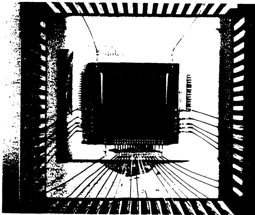
Figure 5.3-3 CCD Array
