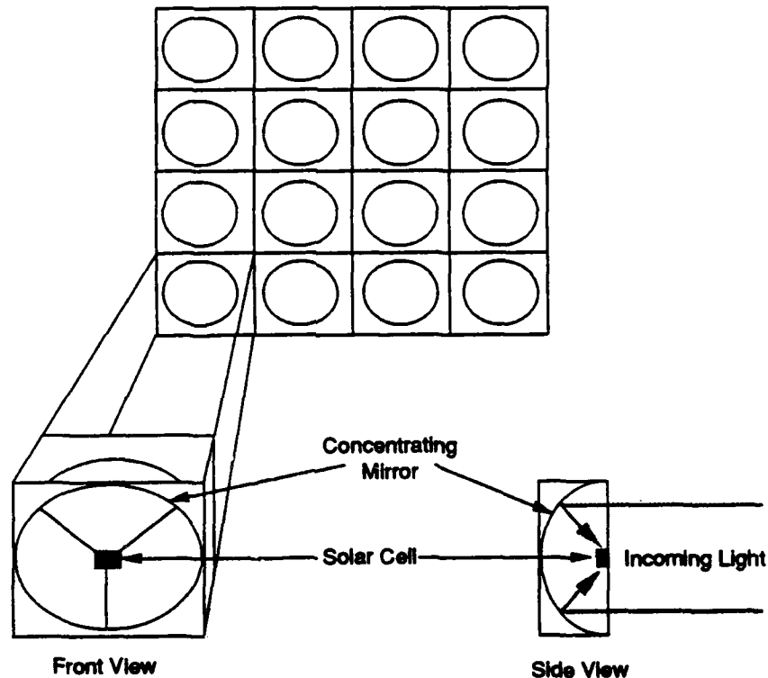
Figure 6.5-6 SCOPA Concept
