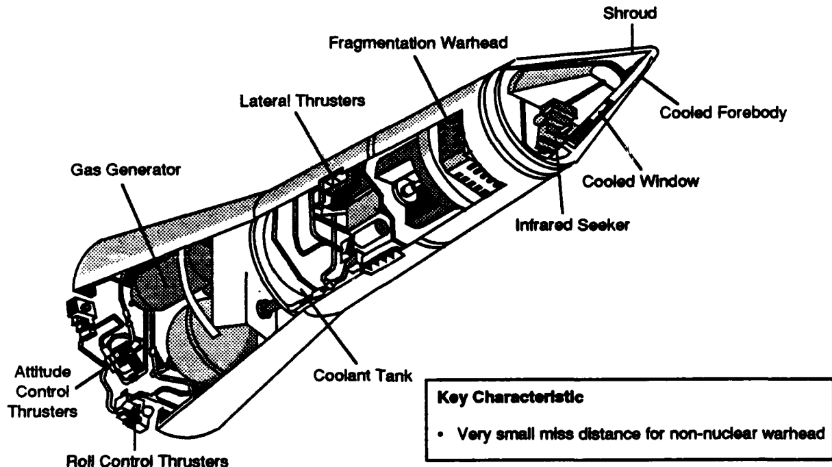
Figure 5.5-1 HEDI Concept
