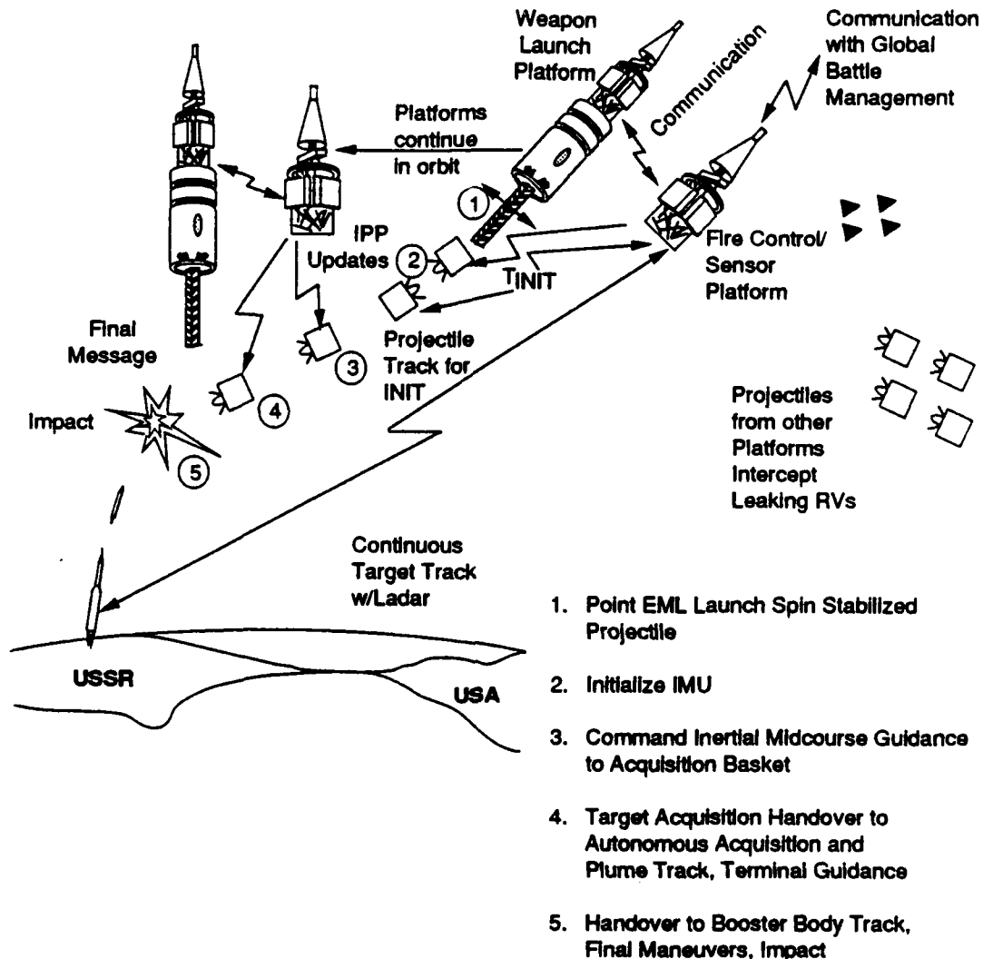
Figure 5.5-6 Space-Based HVG Concept
