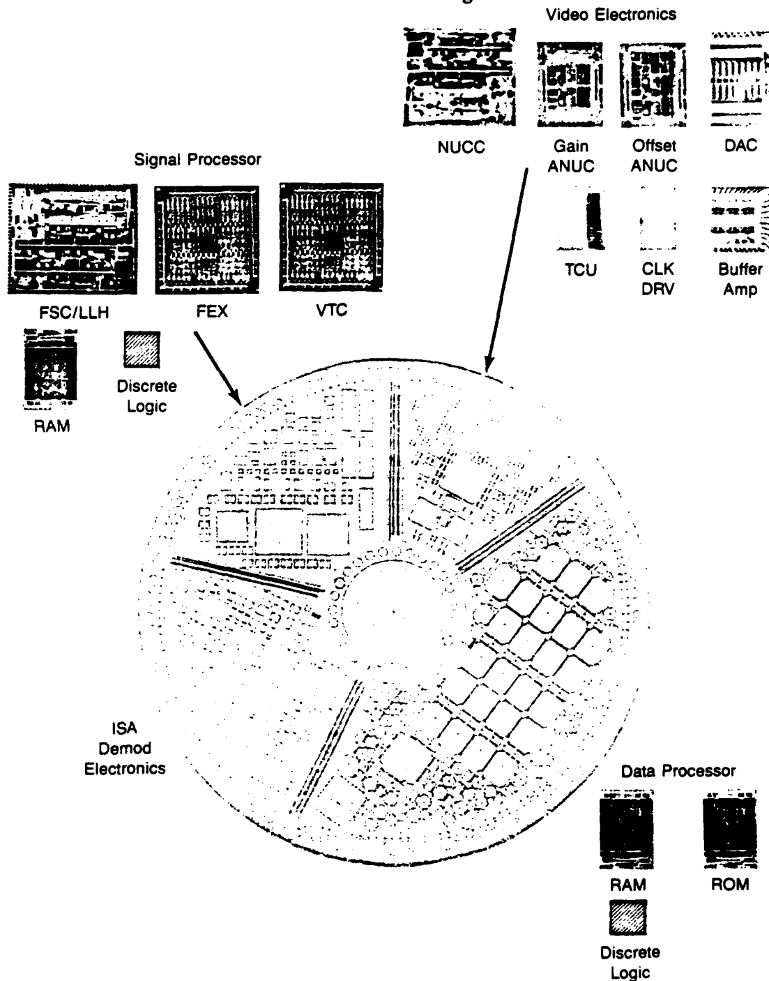
Figure 6.3-4 LEAP Wafer-Scale Integration
