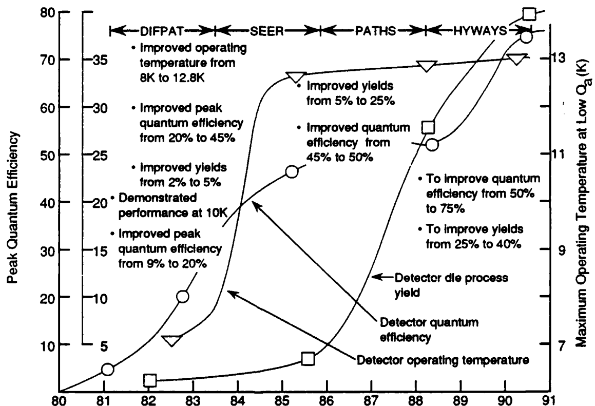
Figure 6.1-4 Si:As IBC Detector Development
