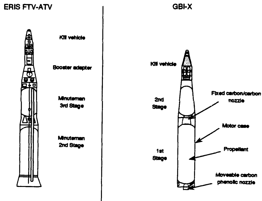
Figure 5.3-9 ERIS FTV-ATV vs. GBI-X
