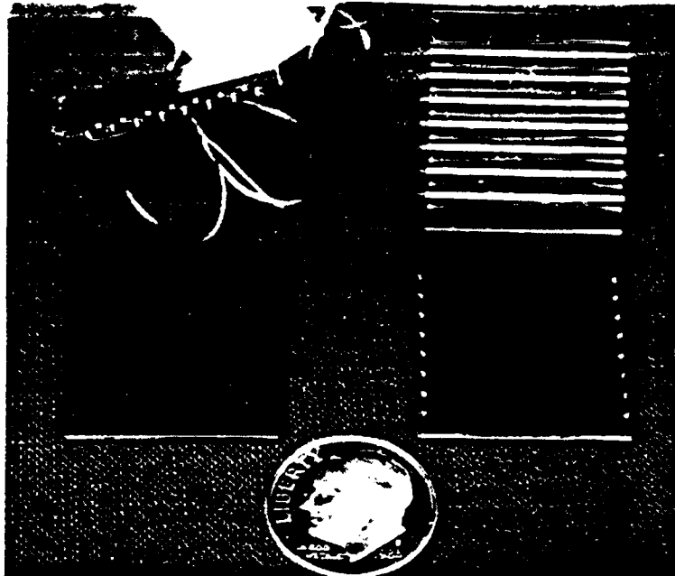
Figure 6.1-9 Millimeter Wave/Ferrite Phase Shifter Array
