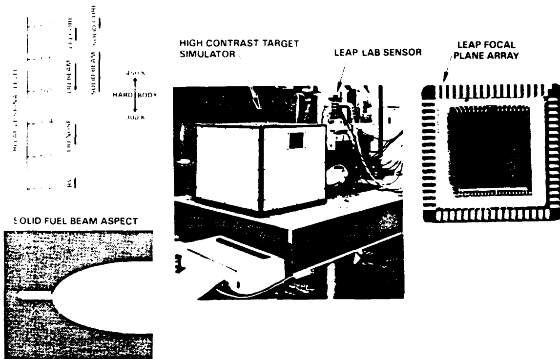
Figure 6.3-3 LEAP 128 x 128 Seeker
