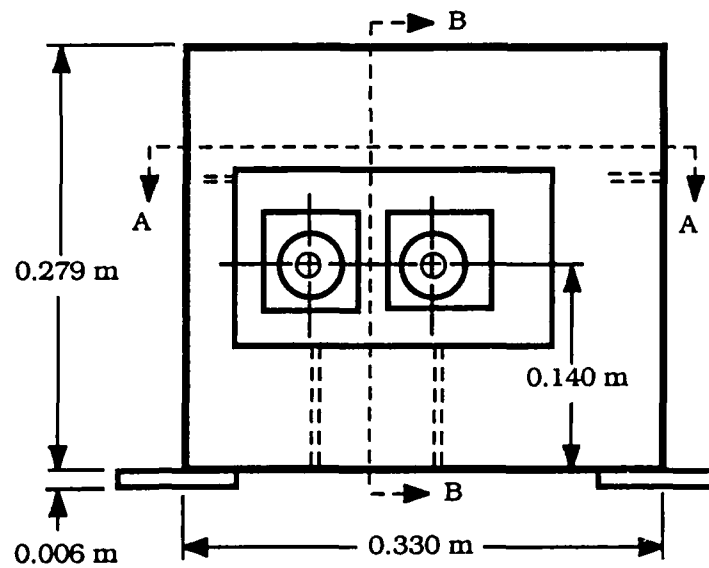
FIGURE 4. - SCHEMATIC OF THE NASA GEARBOX.
