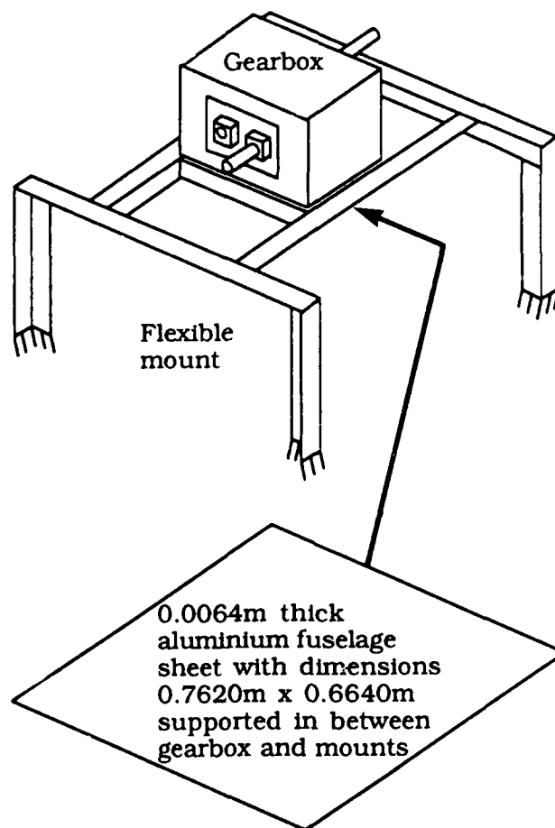
FIGURE 2. - GEARBOX ON FLEXIBLE MOUNTS.
