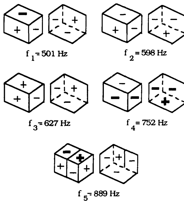
FIGURE 6. - MODE SHAPES OF THE RIGIDLY MOUNTED, STIFFENED NASA GEARBOX SHOWN IN FIGURE 4. BOLD SIGN IMPLIES LARGER AMPLITUDE. ACTUAL BOX ORIENTATION IS THE SAME AS SEEN IN FIGURE 5.
