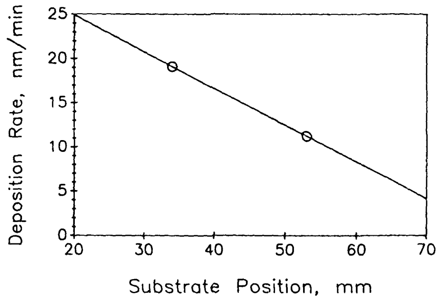
Figure 7. The influence of the center-to-center separation of the target and substrate on deposition rate.
