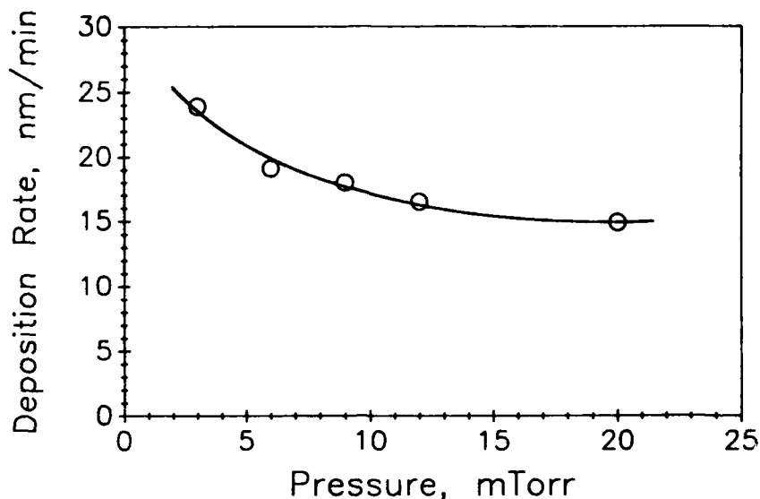
Figure 9. The effect of sputter chamber pressure on the growth rate of as-deposited films.
