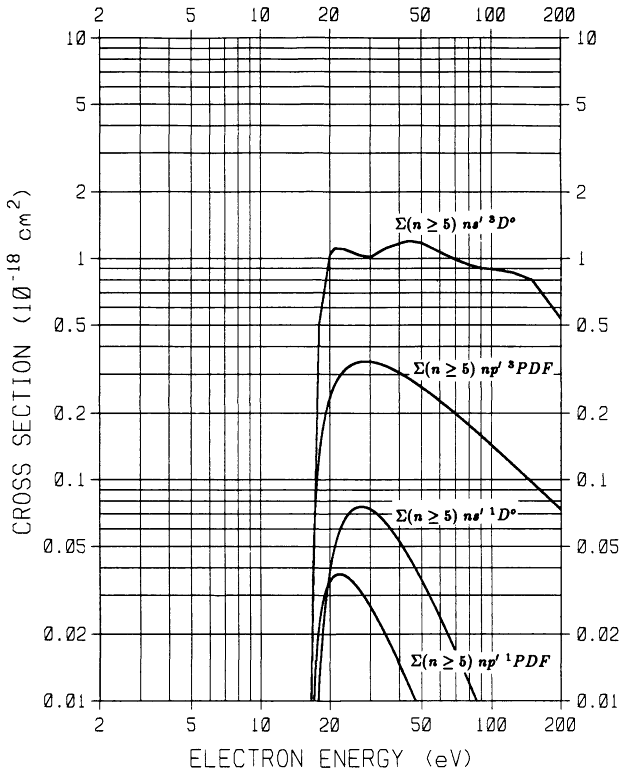
Figure 14. O(^3P \rightarrow \Sigma(n \geq 5) ns' ^3D^\circ, \Sigma(n \geq 5) ns' ^1D^\circ, \Sigma(n \geq 5) np' ^3PDF, \Sigma(n \geq 5) np' ^1PDF) excitation cross sections.
