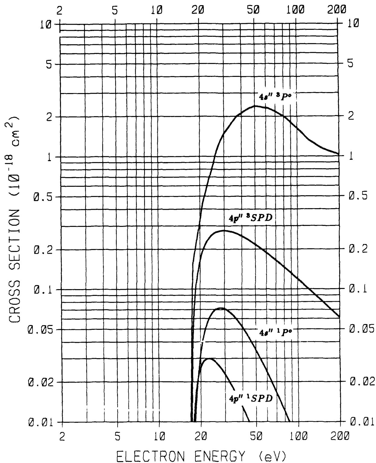
Figure 19. O(^3P \rightarrow 4s'' \ ^3P^\circ, 4s'' \ ^1P^\circ, 4p'' \ ^3SPD, 4p'' \ ^1SPD) excitation cross sections.
