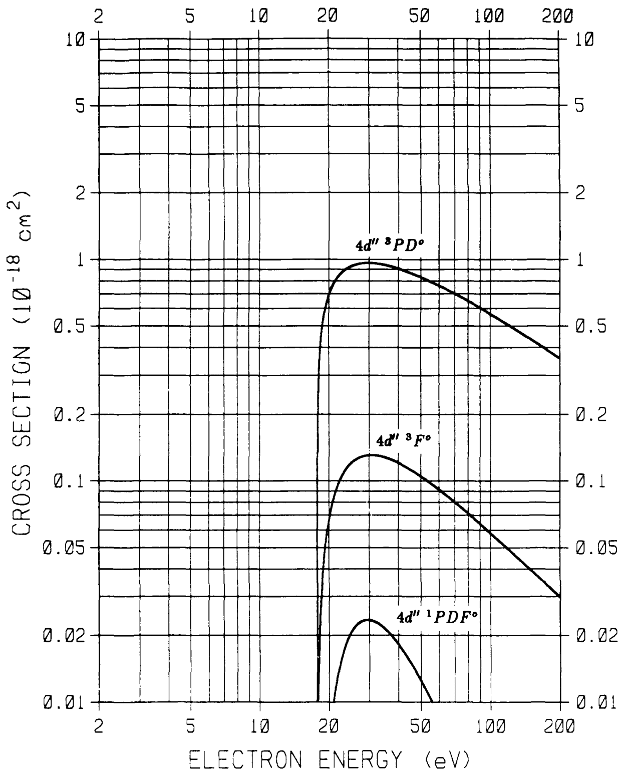
Figure 20. O(^3P \rightarrow 4d'' \text{ } ^3PD^\circ, 4d'' \text{ } ^3F^\circ, 4d'' \text{ } ^1PDF^\circ) excitation cross sections.
