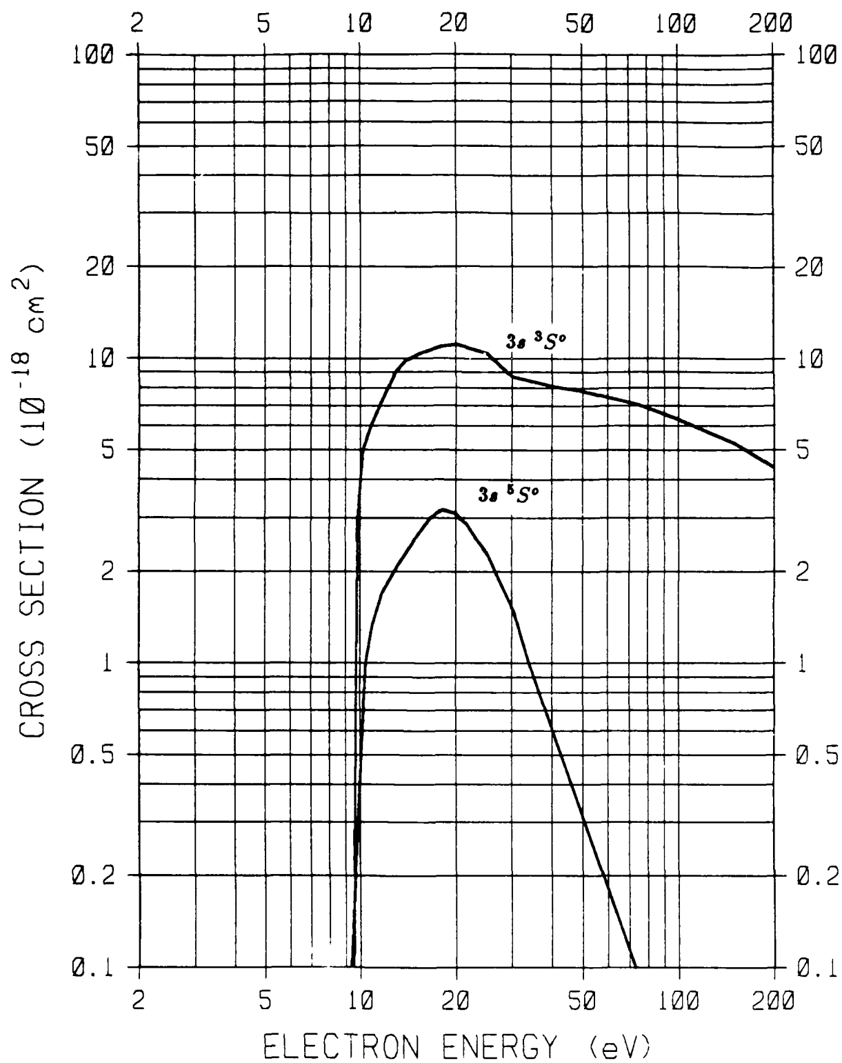
Figure 4. O(^3P \rightarrow 3s\ ^5S^0, 3s\ ^3S^0) excitation cross sections.
