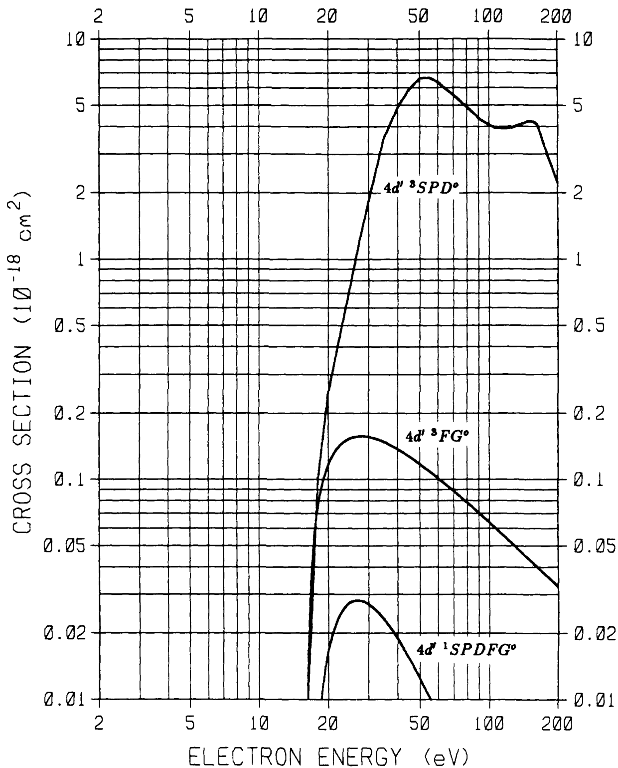
Figure 13. O(^3P \rightarrow 4d' ^3SPD^\circ, 4d' ^3FG^\circ, 4d' ^1SPDFG^\circ) excitation cross sections.
