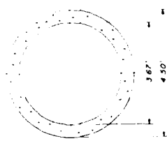
DETAIL - PILE CROSS-SECTION SCALE IN FEET PROTOTYPE 0 1 2
