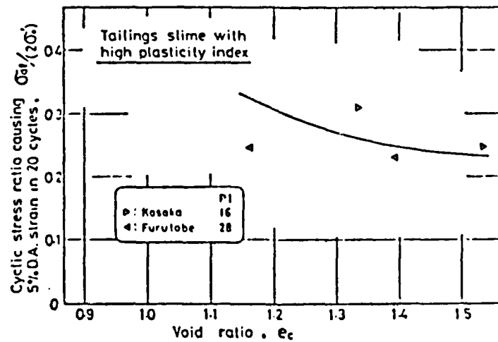
(c) cyclic strength versus void ratio, high plasticity tailings slimes
