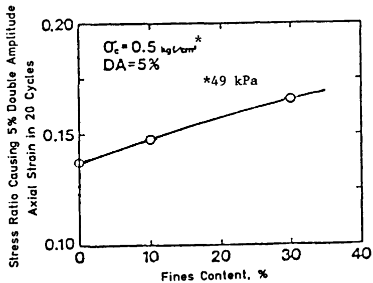
Figure 9. Effect of added fines (kaolin) on cyclic strength of Sengenyama sand at 20 loading cycles (Kondoh, Sasaki, and Matsumoto, 1987)
