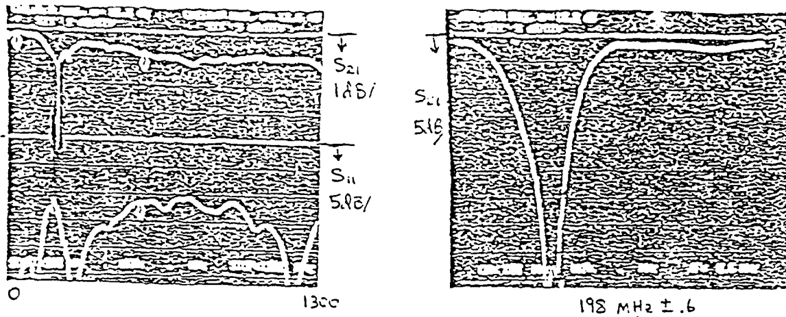
Figure 1.6 Response of prototype bridged-T Filter
