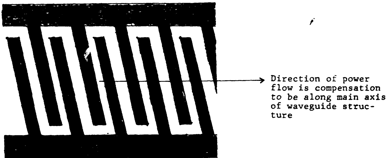
Figure 3.26 Power flow angle compensation.
