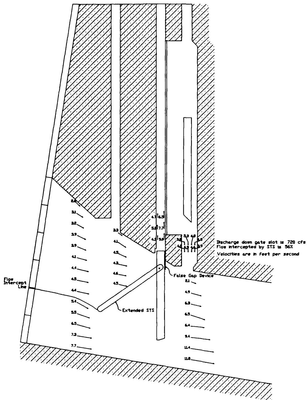
LOWER GRANITE FGE STUDY Test 19 Velocities 55-deg Extended STS Lowered 4 FT False Gap Device Gate Raised 20 FT Pivot EI 632.4
