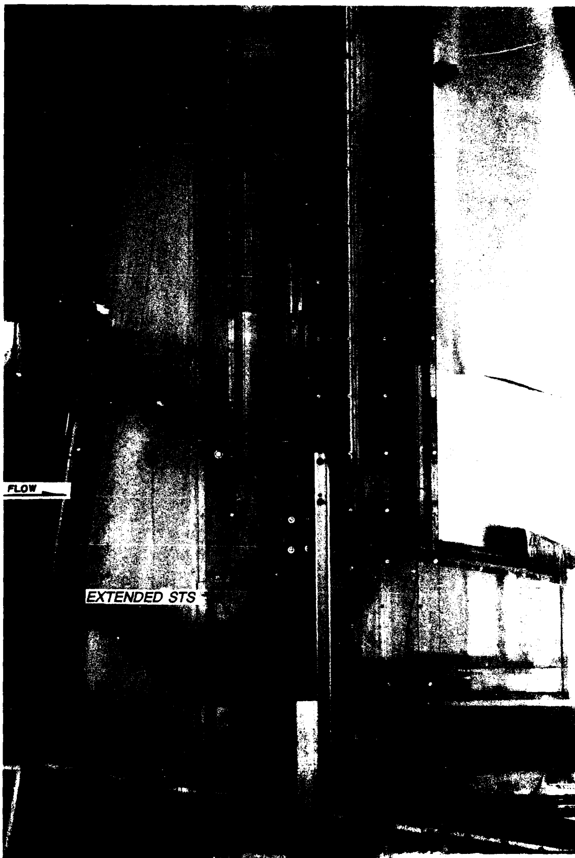
Photo 7. 55-deg extended STS lowered 4 ft with the false gap device in place and the closure gate in its normal position
