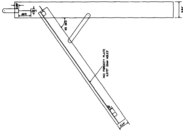
SECTION A-A 65-DEG OPERATING POSITION
