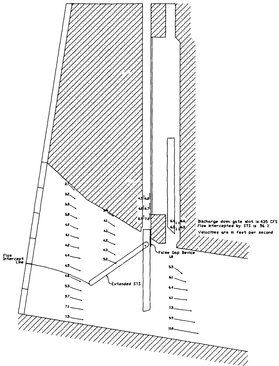
LITTLE GOOSE FGE STUDY Test 35 Velocities 55-deg Extended STS Lowered 4 FT False Gap Device Gate Raised 5 FT Pivot EI 632.4
