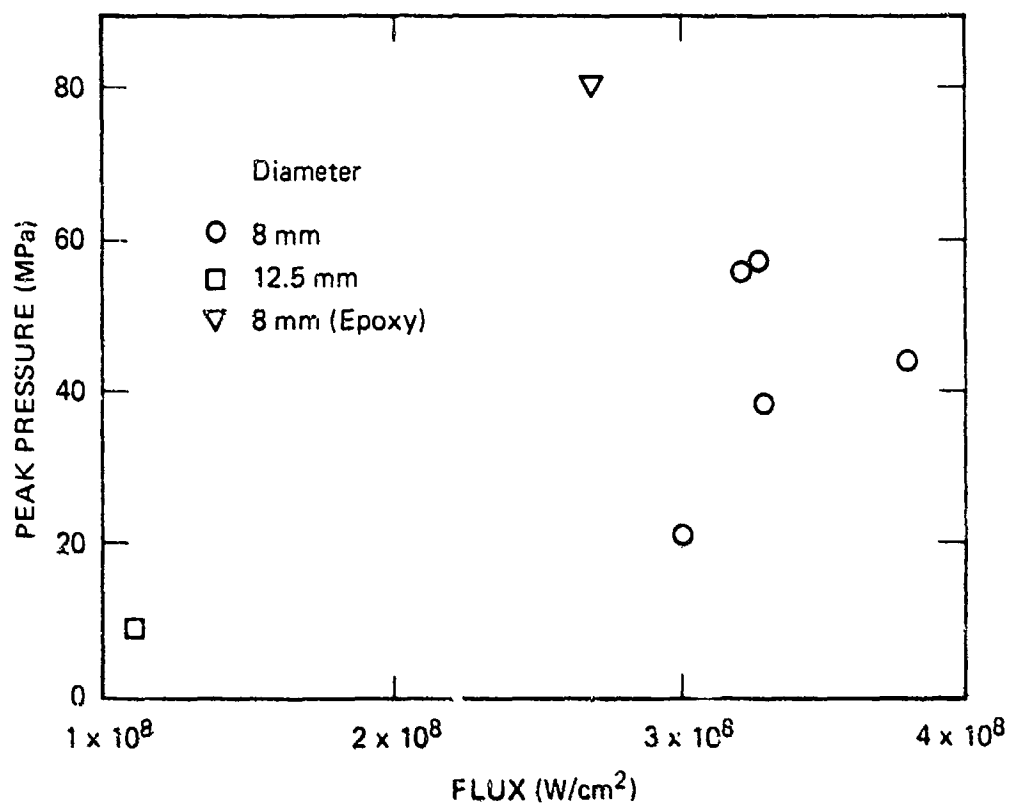
Figure 24. Peak pressure as a function of flux.
