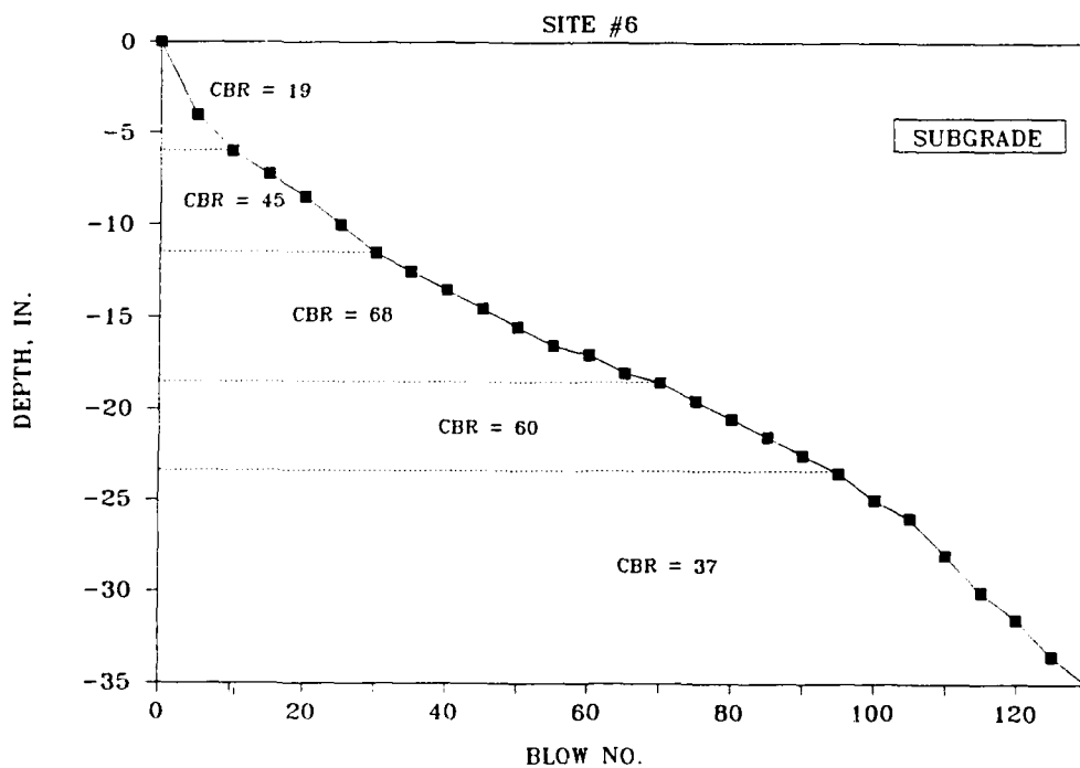
Figure 25. DCP results (Site 6)
