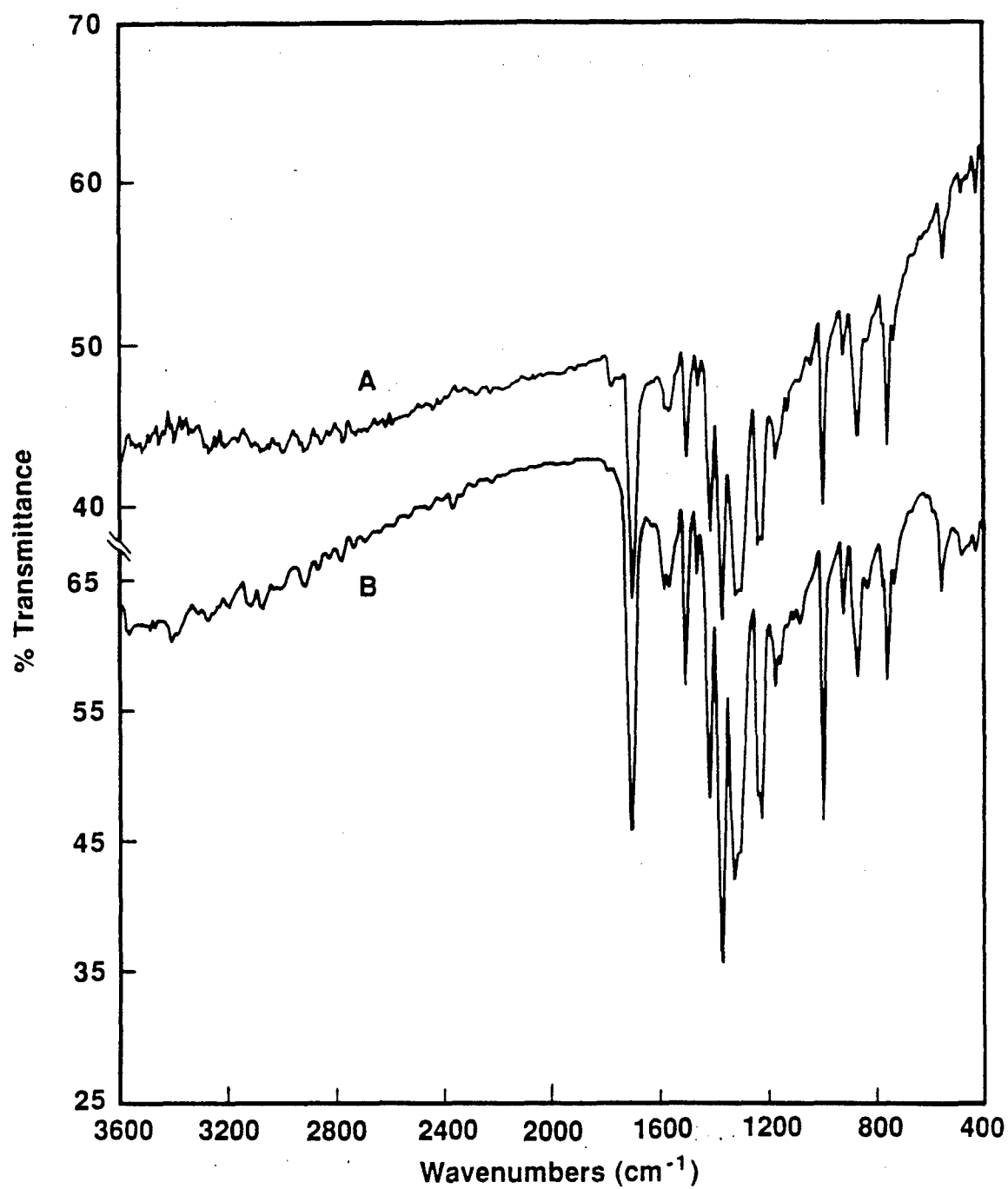
FIGURE 23 FTIR spectra of BBL thin films: A -- pristine polymer; B -- polymer regenerated from a \text{FeCl}_3/\text{CH}_3\text{NO}_2 solution.
