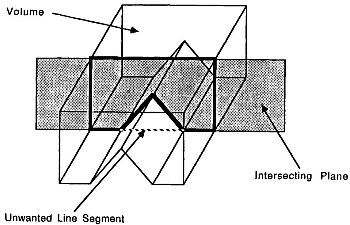
Figure 23. Non-Convex Intercept
