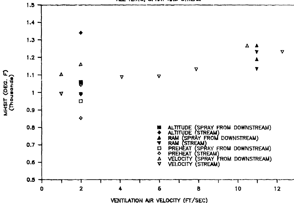
Figure 58. 7808 Correlation Based on a Simplified Expression of Ignition Delay and Translt Time
