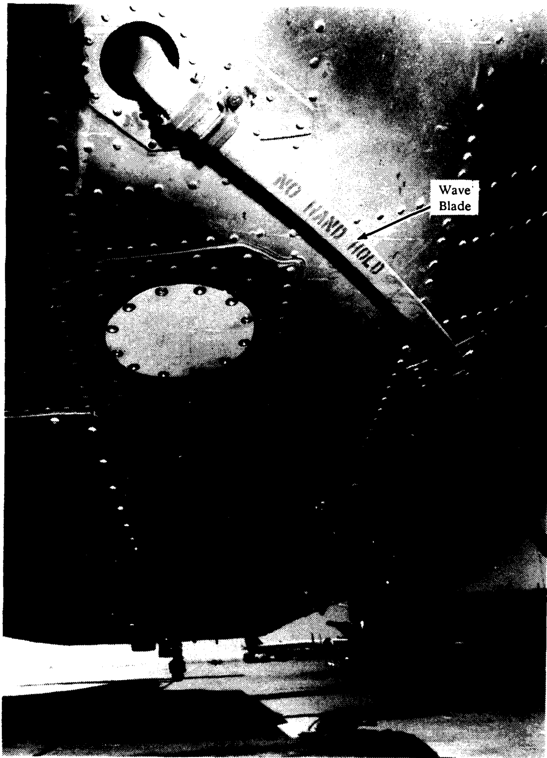
Figure B-22. Forward Bottom View AN/ALQ-162 Wave Guide Installation
