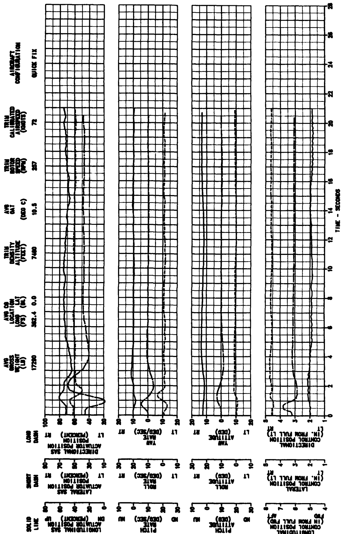
FIGURE E-46 DIRECTIONAL PULSE INPUT EH-60A USA S/N 86-24500
