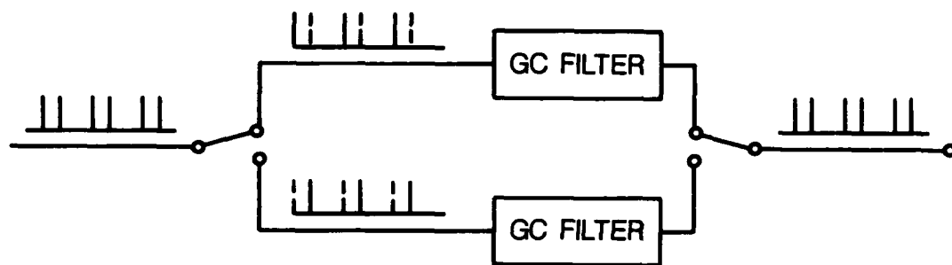
Figure 3. Ground clutter filter consisting of a pair of filters, each of which is for a low-PRT uniform pulse train. This pair is referred to as the split uniform PRT ground clutter filter.
