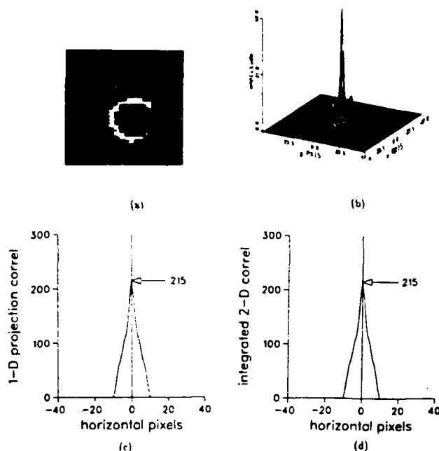
Fig. 3. Comparison of a projection correlation and an integrated 2-D correlation: (a) input character C image; (b) 2-D correlation; (c) vertical projection correlation; and (d) vertically integrated 2-D correlation.
