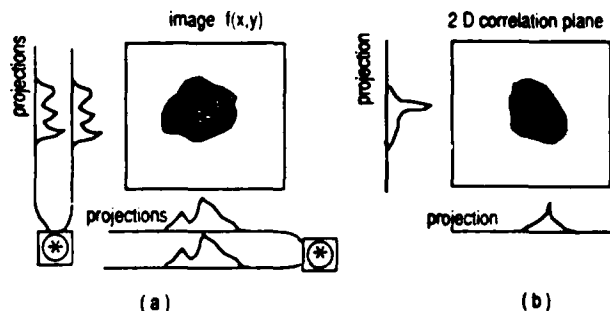
Fig. 2. Equivalence of 1-D projection correlations and projections of the 2-D correlation pattern: (a) horizontal and vertical projections of a 2-D image; (b) horizontal and vertical projections of the 2-D correlation pattern.
