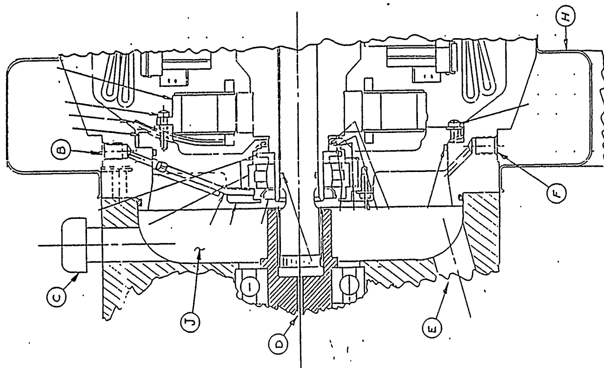
FIGURE 3. ALTERNATOR / GEARBOX / TYPICAL INSTALLATION
