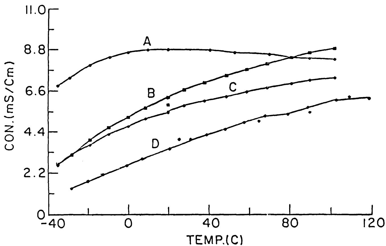
Fig. 9. Conductivity of 0.84M BaX 2 -TC-SO 2 solutions vs temperature. SO 2 volume percent: A-40; B-20; C-10; D-0.
