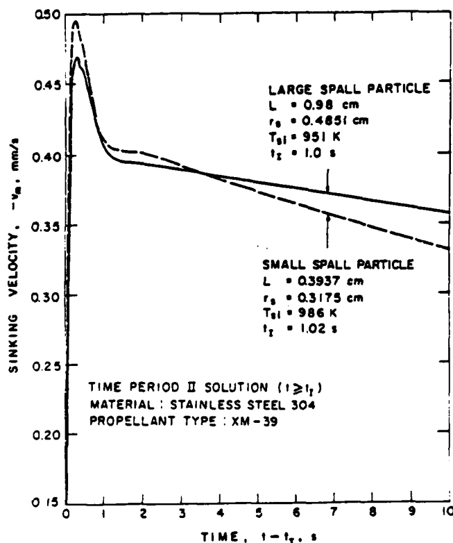
Fig. 15 Calculated Time Variations of Sinking Velocity
