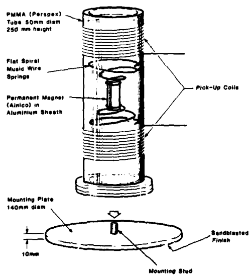
FIGURE 5 Schematic diagram of a velocity gauge.
