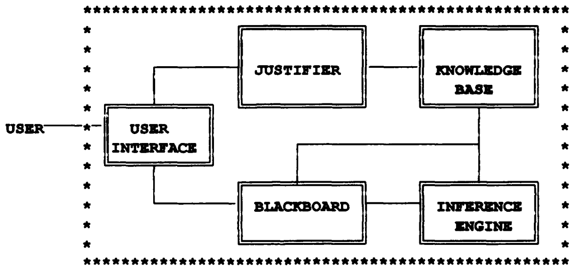
Figure 2.8 ES Structure
