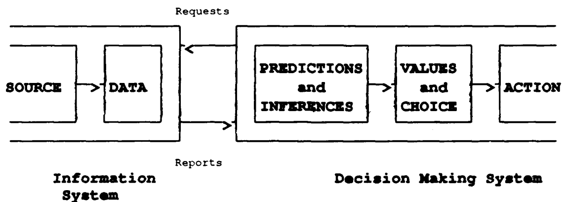
Figure 2.2 Database System
