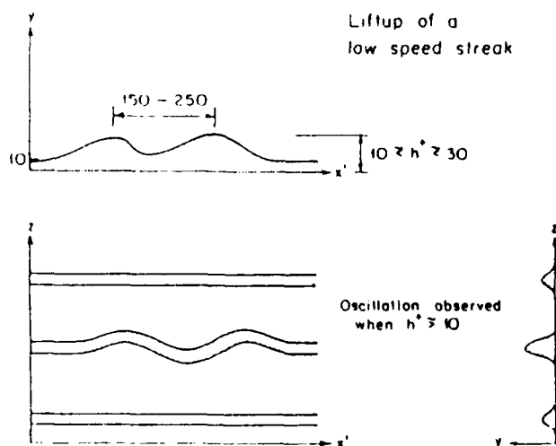
Figure 5. Sketch of the lift-up of a portion of the LSS.
