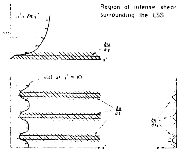
Figure 4. Sketch of the low speed streaks (shaded areas) showing the regions of intense shear surrounding the low speed fluid. The inflectional surface is embedded within the strong shear region.
