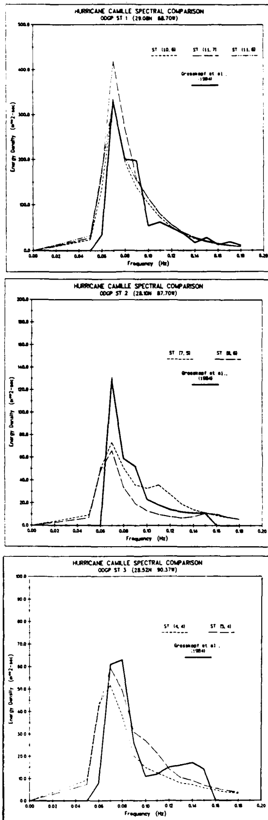
Figure D5. Comparison of measured and modeled wave spectra for maximum wave conditions during Hurricane Camille at three different sites
