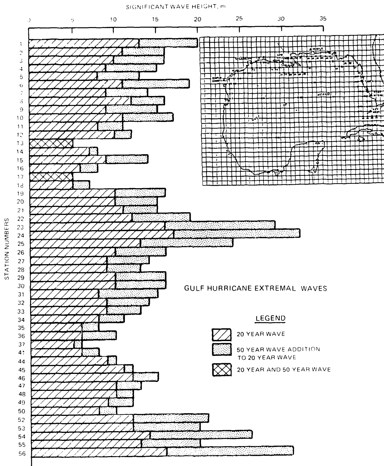
Figure 20. The 20- and 50-year wave heights for all gulf stations
