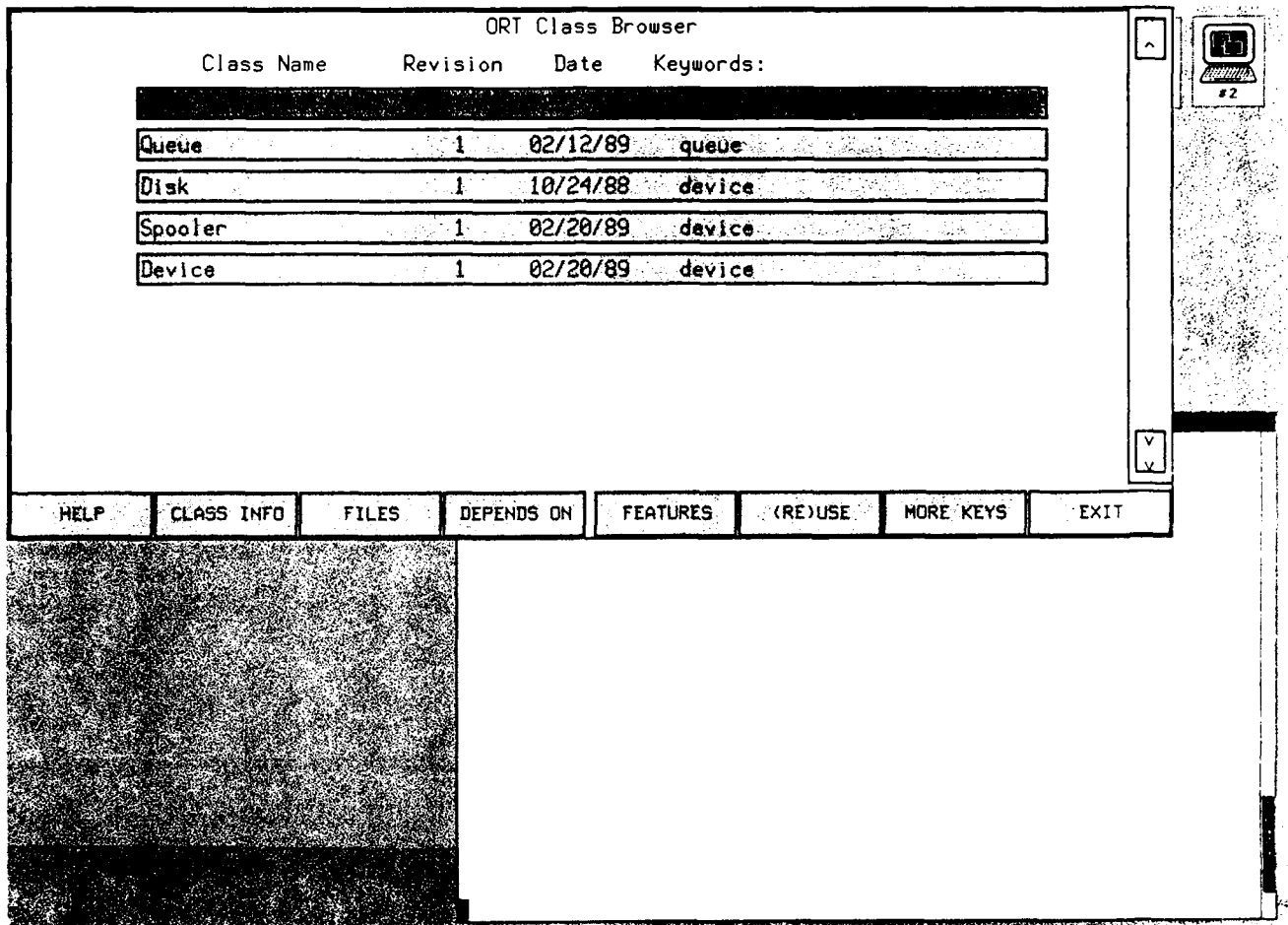
Figure 6-2: Class browser containing relevant candidates for "Node".
