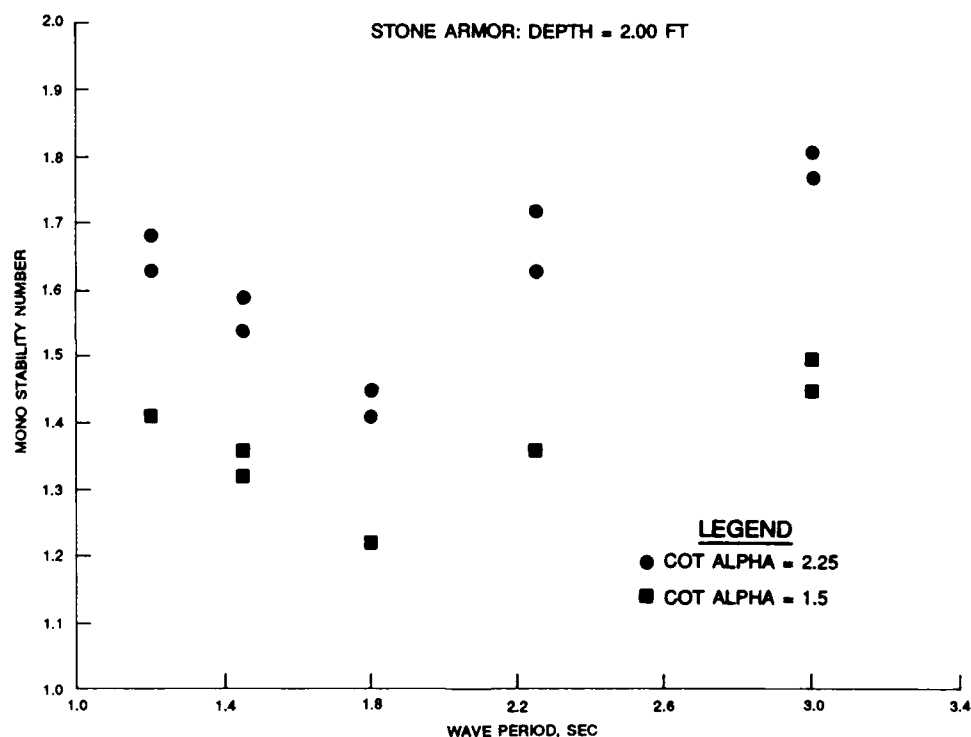
Figure 4. Monochromatic stability number versus wave period
