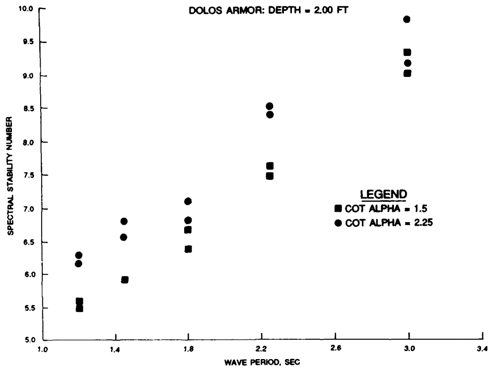
Figure 8. Spectral stability number versus period
