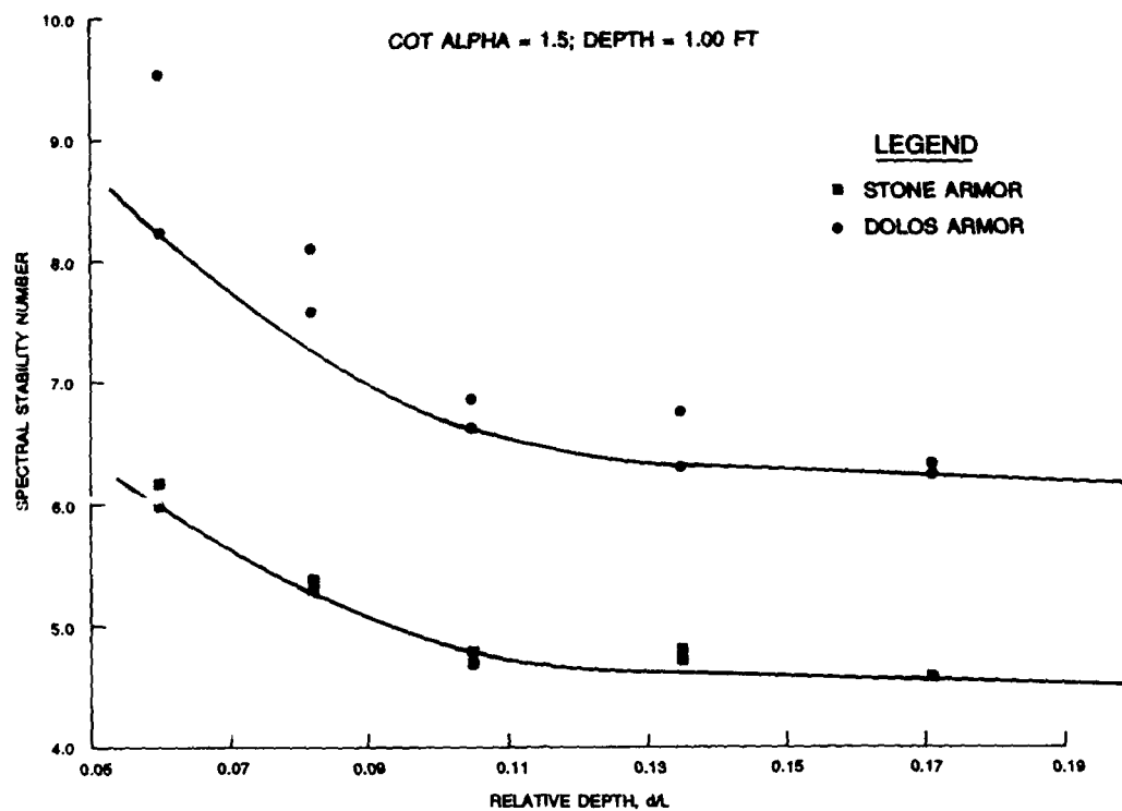
Figure 12. Spectral stability number versus d/L number and relative wave height. However, effects of this variable appear to be minor relative to the influences of wave period and breakwater slope. Influences of H_{mo}/d can be accounted for by using Figures 6 and 9 when H_{mo}/d is less than 0.21, and Figure 12 may be applied if H_{mo}/d is greater than 0.34. If 0.21 < H_{mo}/d < 0.34 , both curves should be checked and the stability number yielding the larger armor weight used.
