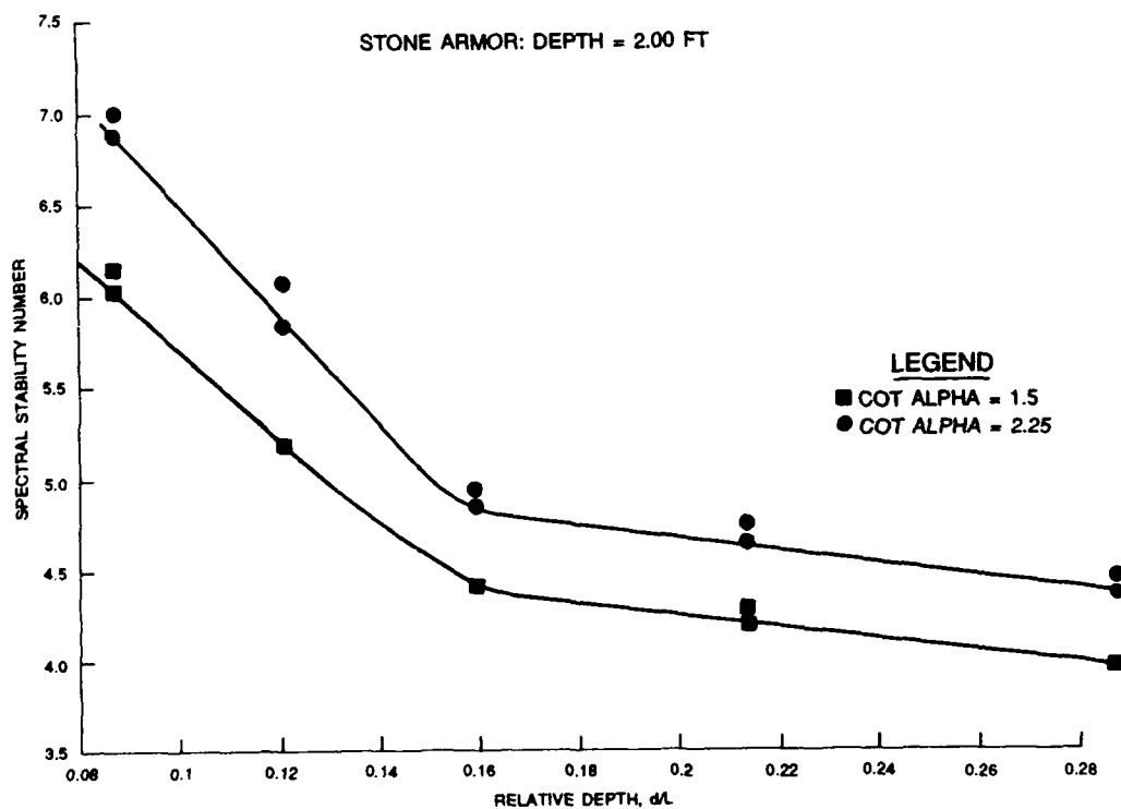
Figure 6. Spectral stability number versus d/L
