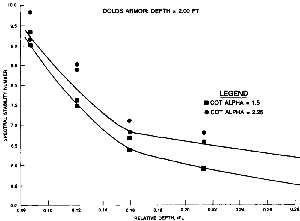
Figure 9. Spectral stability number versus d/L
