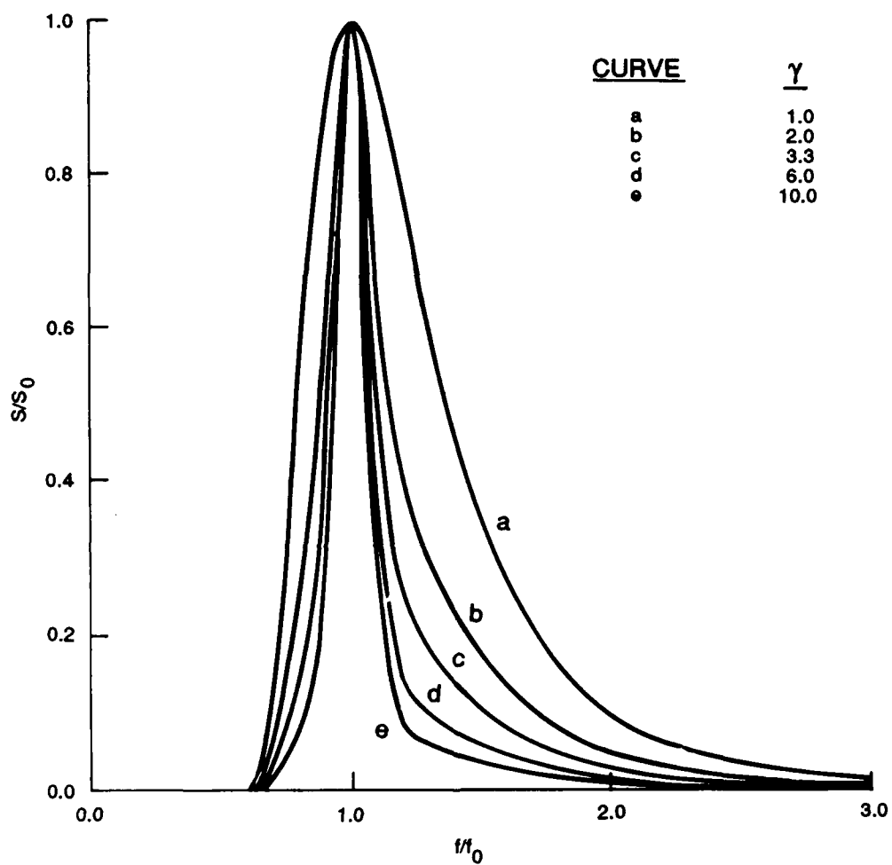
Figure 1. Five examples of JONSWAP spectra in dimensionless form (curve a is a Pierson-Moskowitz spectrum; curve c is the result of the JONSWAP experiment)
