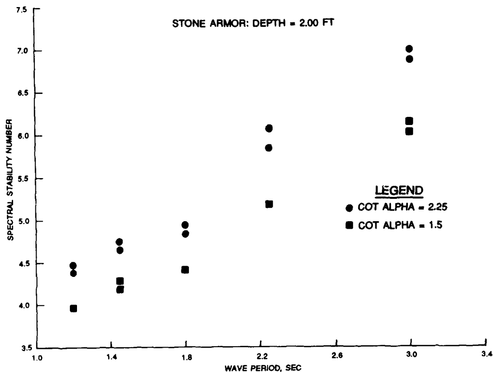
Figure 5. Spectral stability number versus period response. Therefore, N_{spec} is plotted as a function of d/L in Figure 6, and a strong correlation is observed.
