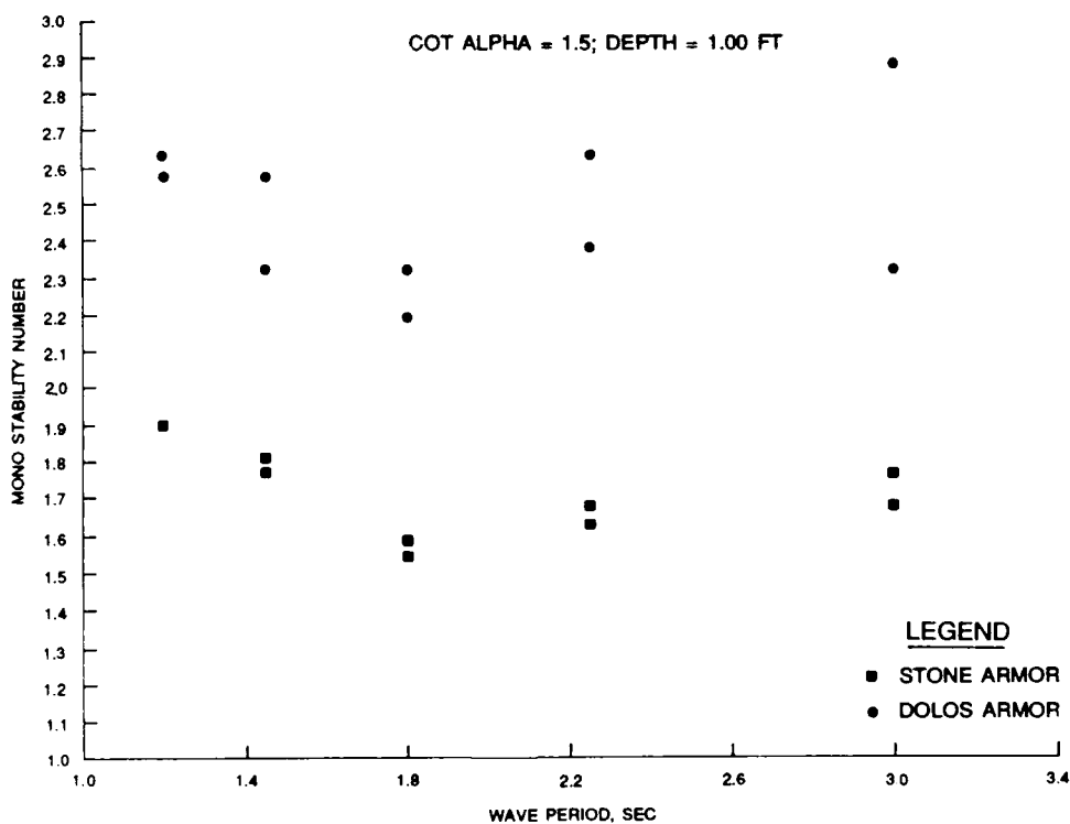
Figure 10. Monochromatic stability number versus wave period
