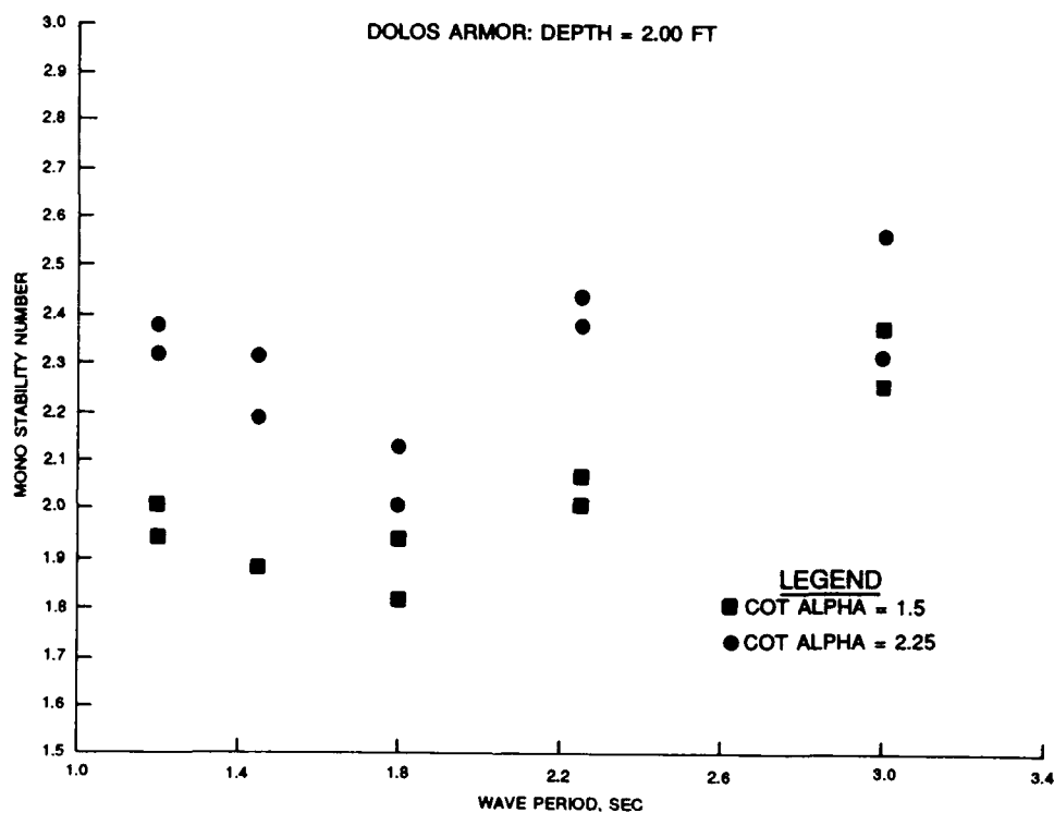
Figure 7. Monochromatic stability number versus wave period
