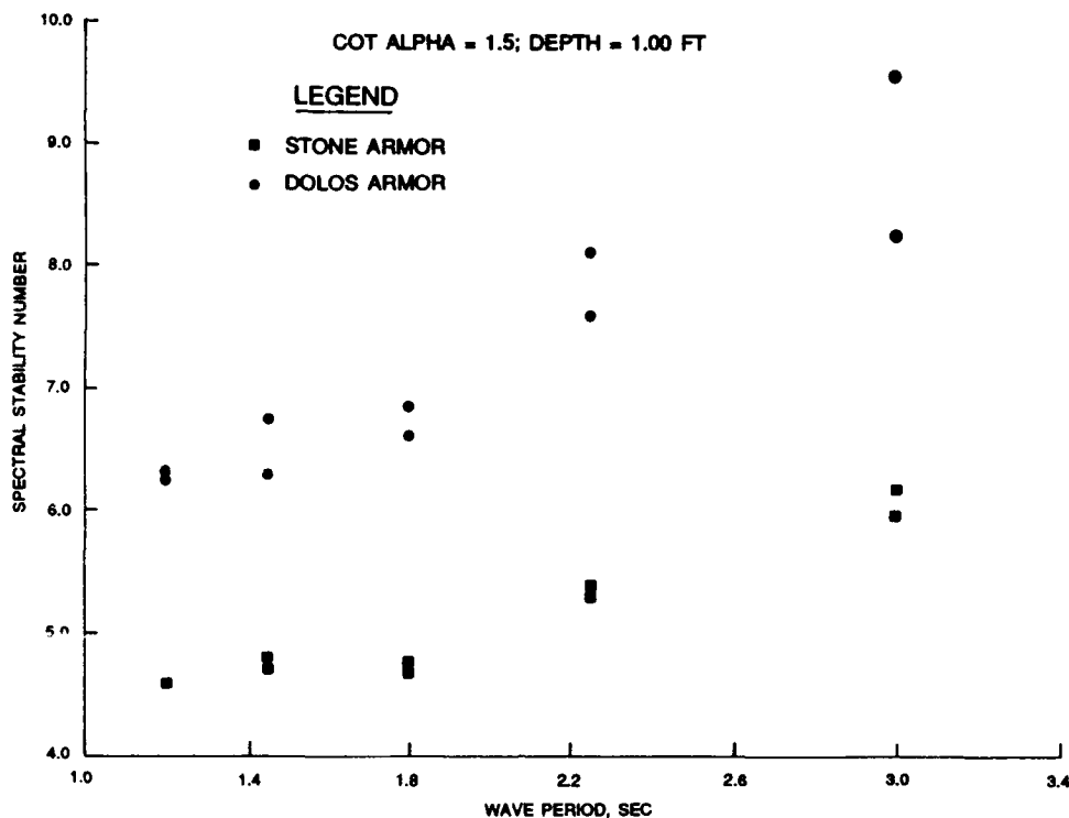
Figure 11. Spectral stability number versus period
