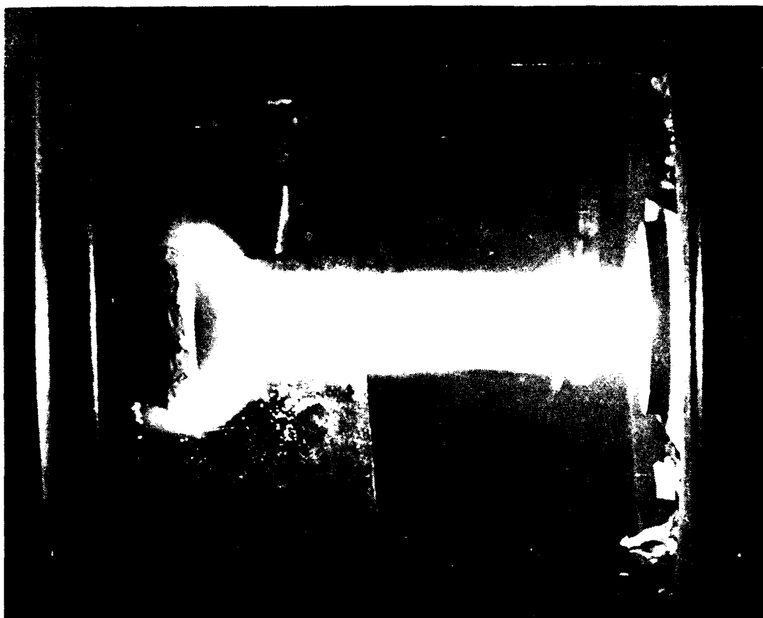
Fig. 5. Subsonic arc jet convection heating test of EPDM sample ( 84 \text{ Btu ft}^{-2} \text{ sec}^{-1} centerline heating rate).
