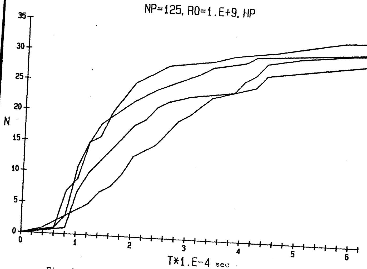
Fig. 5 - Number of collisions particle size (ii), initial concentration (i)
