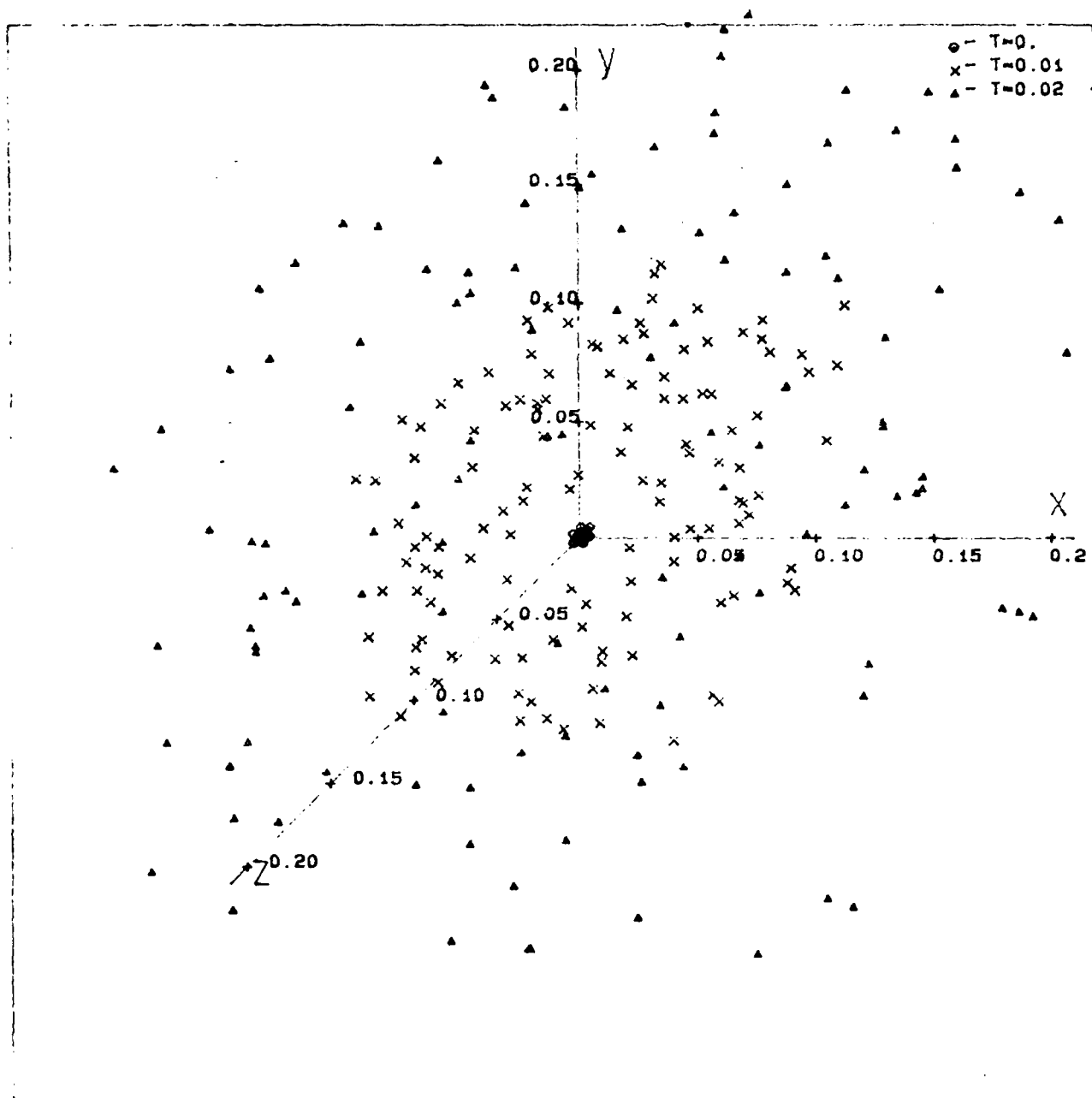
Fig. 3 - 3-D Dispersion
